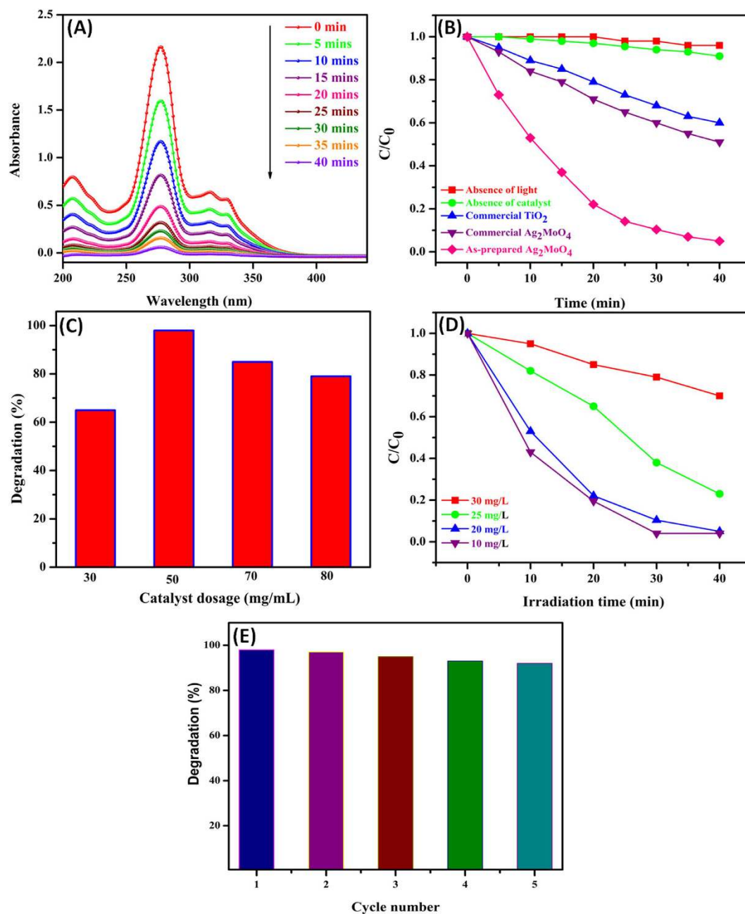
Figure 7. (A) Absorption spectrum of CIP in the presence of 50 mg/mL Ag 2 MoO 4 under UV-light illumination. (B) Photodegradation of CIP in the presence of different catalysts. (C) Effect of catalyst amount dosage on the photodegradation of CIP. (D) Effect of initial CIP concentration on the photodegradation and (E) reusability of the potato-like Ag 2 MoO 4 photocatalyst.
