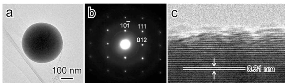
Figure 4 | TEM images and diffraction pattern of a fabricated ZnSe microsphere. (a) Typical TEM image of a ZnSe microsphere. (b) Electron diffraction pattern of the ZnSe microsphere shown in (a) taken along the [-12-1] zone axis. (c) High-resolution TEM image of the sphere shown in (a).
