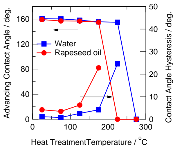
Fig. 8. Change in the advancing contact angle and contact angle hysteresis for water and rapeseed oil of the FAP-coated dual-pore surface, chemically etched in solution containing 1 \text{ mol dm}^{-3} HCl, anodized and pore-widened for 1200 s, with heat treatment temperature.
