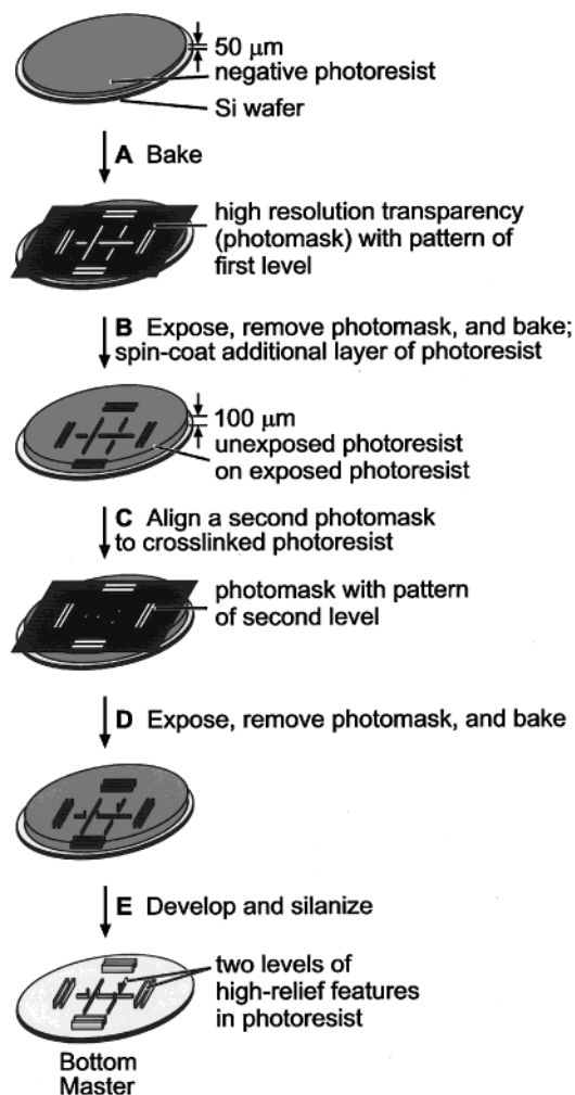
Figure 1. Scheme describing the fabrication of the bottom master of two levels of photoresist on silicon by multilevel photolithography. (A) A layer of negative photoresist, 50–150 \mu\text{m} thick, was spin-coated on a silicon wafer and soft-baked for 5–15 min. (B) A high-resolution transparency containing the lowest level of the channel system and alignment tracks was used as the mask in photolithography. The photoresist was hard-baked and a second layer of negative photoresist, also 50–150 \mu\text{m} thick, was spin-coated on top of the first. (C) A second high-resolution transparency was aligned to the exposed features under the unexposed photoresist. This transparency contained the design for the middle level of the channel system (the interconnects between channels in the lowest and uppermost levels) as well as the alignment tracks. (D) The resist was exposed and soft-baked for 10–20 min. (E) The master was developed to yield two levels of high-relief features and passivated by vapor-phase silanization.
