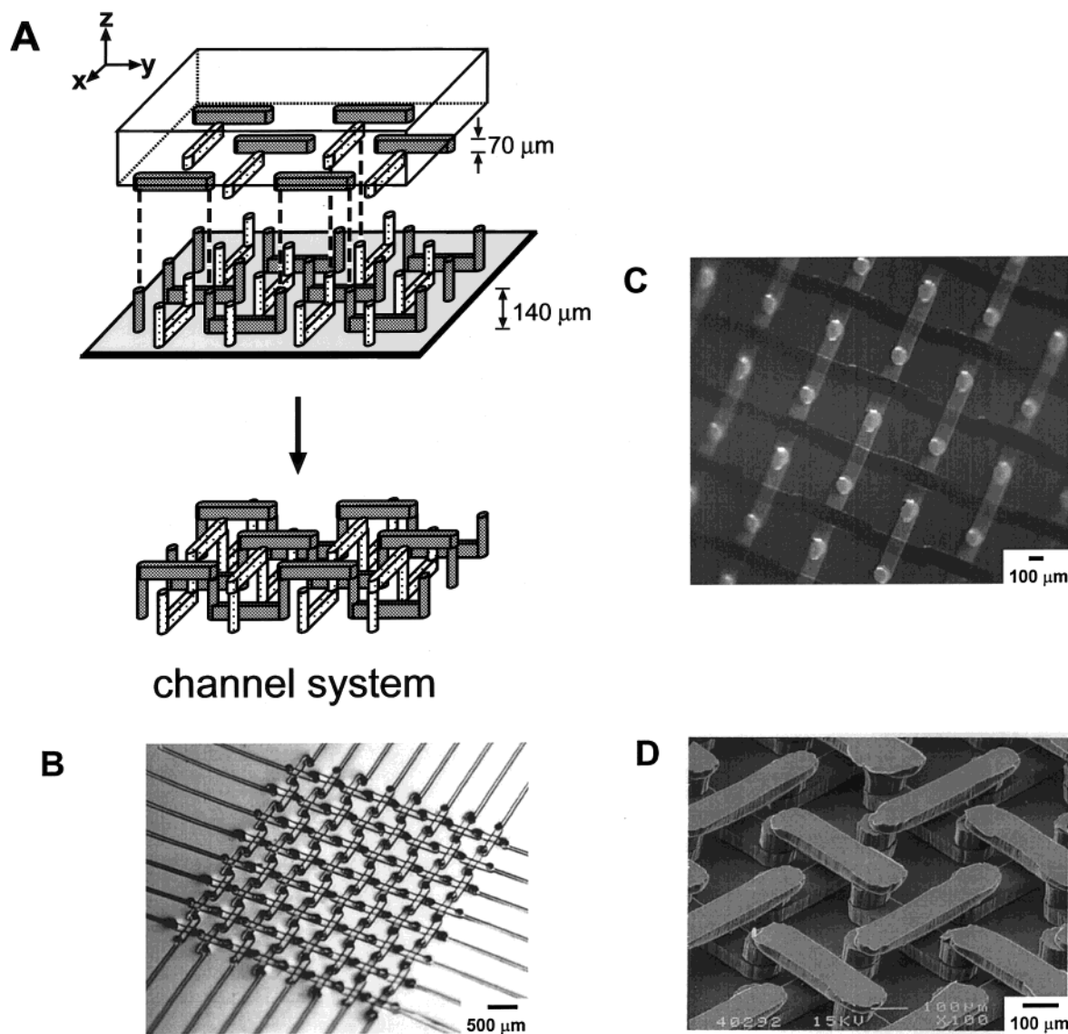
Figure 4. A microchannel system in a basketweave pattern. (A) Schematic illustration of a portion of the structure of top and bottom masters and the channel system that results from using them in a membrane sandwich. For clarity, features in photoresist oriented in the y -direction are depicted with a darker pattern than those in the x -direction. (B) Optical micrograph (looking down the z -axis) of the PDMS membrane alone, which contains the entire 8 \times 8 channel system. The channels are 100 \mu\text{m} wide ( x - or y -direction), and each of the three levels used in the fabrication is 70 \mu\text{m} high ( z -direction) but is not enclosed. (C) Optical micrograph (looking down the z -axis) of a portion of the enclosed, fluid-filled channels. Channels in the y -direction are filled with a solution of fluorescein and channels in the x -direction are filled with a solution of Meldola's Blue dye. (D) Scanning electron micrograph of the microstructure in epoxy polymer. It was formed by filling the basketweave channel system with epoxy prepolymer, curing under ultraviolet light for 10 min, and dissolving the PDMS casing in tetrabutylammonium fluoride.
