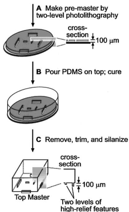
Figure 2. Scheme describing the fabrication of the top master of PDMS by replica molding. (A) Multilevel photolithography was used to generate a pre-master: two levels of low-relief features in a photoresist layer on a silicon wafer. The shallow level went only halfway through the double layer of photoresist (100–300 \mu\text{m} thick in total); it included features for the uppermost level of the channel system. The deeper level went through the entire double layer of photoresist to the silicon surface and included no part of the channel system, only the alignment track. (B) Prepolymer of PDMS was poured onto the pre-master and cured at 75 ^{\circ}\text{C} for 1 h. (C) The PDMS was peeled off the pre-master, trimmed to a convenient size, oxidized for 1 min in an air plasma, and passivated by vapor-phase silanization to give the top master of PDMS with high-relief features.
