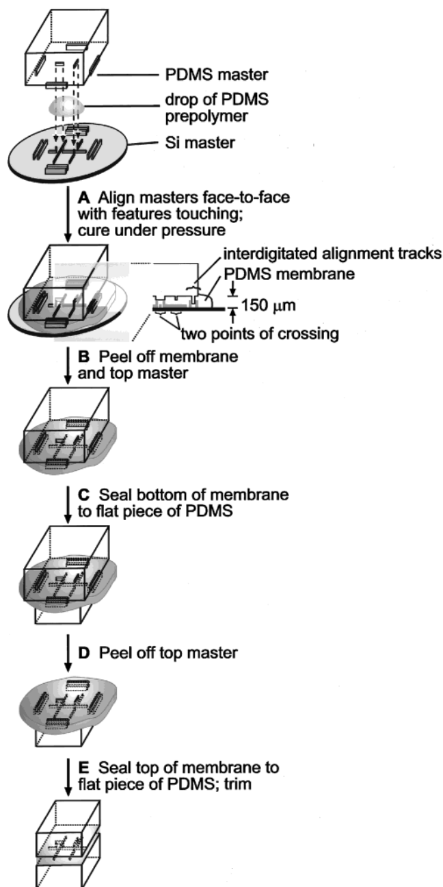
Figure 3. Scheme describing the membrane sandwich method. (A) The top master was placed facedown on top of the bottom master with a drop of PDMS prepolymer in between. The top master slid on the prepolymer until its tall alignment track fell into the tall alignment tracks of the bottom master and the segments of the channel system from both masters were aligned. Sufficient pressure was applied to the top master so that prepolymer did not seep between features that were in contact, and the PDMS was heated to 75 °C and cured in place. (B) The PDMS membrane and the top master were peeled off the bottom master. (C) The bottom of the membrane and a flat slab of PDMS were oxidized in an air plasma for 1 min and brought into contact to seal. (D) The top master was peeled off. (E) The top surface of the membrane was sealed to a flat slab to enclose the channel system and trimmed to a convenient size.
