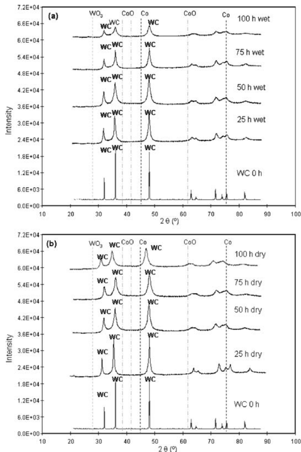
a wet; b dry 7 X-ray diffraction of WC-12Co powders mixture as function of milling time and processing
