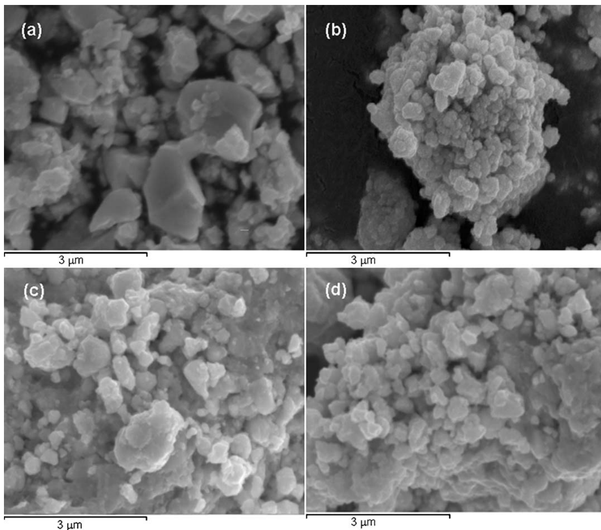
a 25 h, wet milling; b 100 h, wet milling; c 25 h, dry milling; d 100 h, dry milling 1 Images (SEM) of WC-12Co powders after milling
