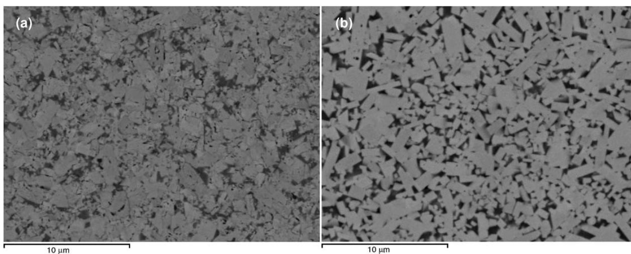
a vacuum at 1400°C for 60 min; b HIP at 1250°C, 1500 MPa for 30 min
