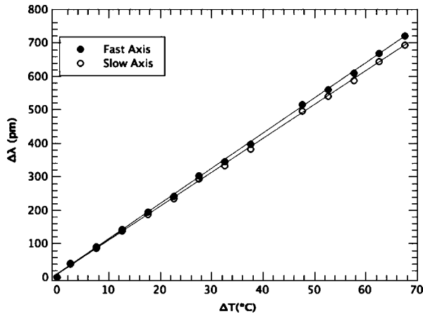
Fig. 7. Sensing head response (two peaks) to temperature.
