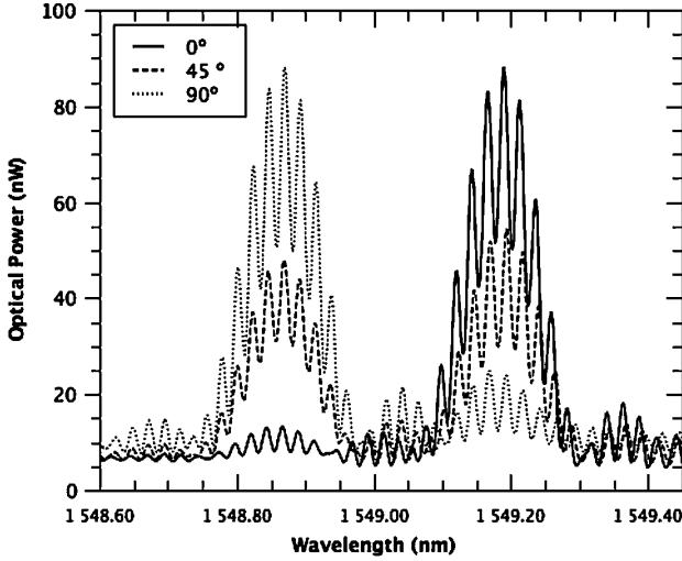
Fig. 3. Channeled spectra for different polarization angles.
