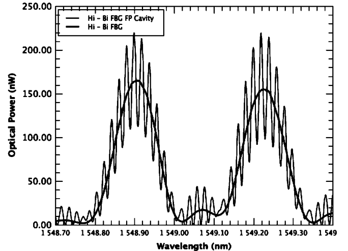
Fig. 2. Hi-Bi FBG before the cavity is created (bold) and Fabry–Pérot cavity spectra obtained after cleaving the fiber end.
