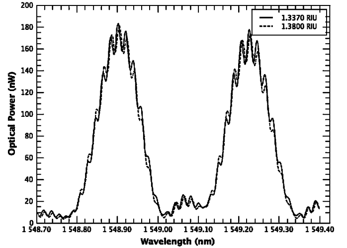
Fig. 5. Channeled spectra for two different RI solutions.
