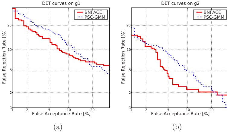
Fig. 3. DET curves obtained on the Mc protocol of the BANCA database for the BNFACE (solid line) and the PSC-GMM (dashed line) models
