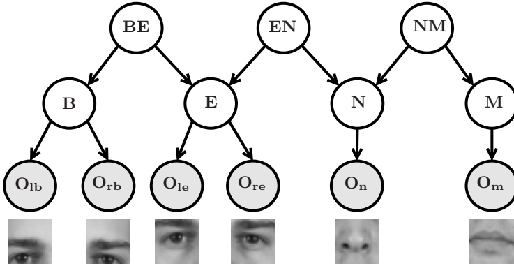
Fig. 1. Static Bayesian Network for Face Representation
