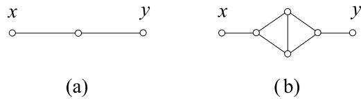
FIG. 1. Replacing vertices of degree 2 in G_1
