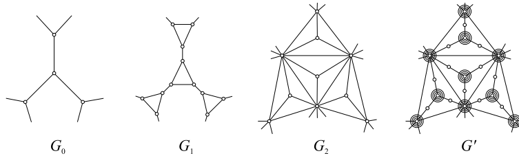
FIG. 3. From G_0 to G'
