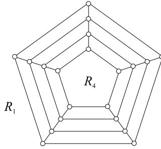
FIG. 2. The graph H_{5,4}
