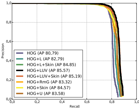
Fig. 8. Quality versus colour channels
