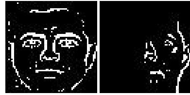
Fig. 2. Example of an image after the DoG filtering stage for the same person under good illumination (left) and bad illumination conditions (right). The bad illumination causes a shadow on the left half of the face preventing DoG filtering from finding the correct edges.
