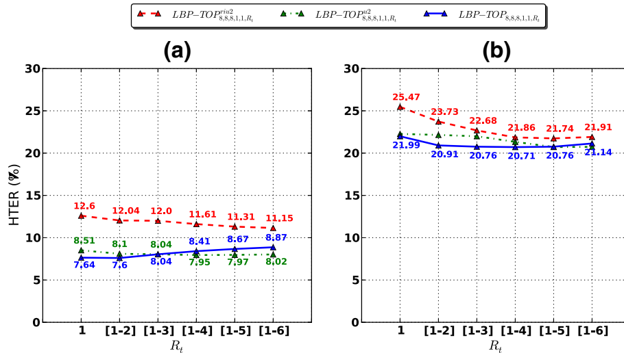
Figure 9 Evaluation of HTER (%) with LBP-TOP 8,8,8,1,1,R t using different LBP configurations in planes with SVM classifier. (a) Replay-Attack Database (b) CASIA Face Anti-Spoofing Database.
