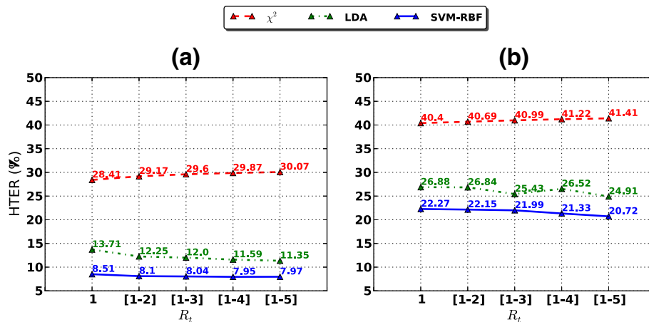
Figure 8 Evaluation of HTER (%) with LBP-TOP 8,8,8,1,1,R t u2 using different classifiers. (a) Replay-Attack Database. (b) CASIA Face Anti-Spoofing Database.
