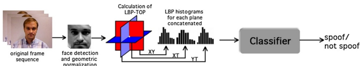
Figure 3 Block diagram of the proposed countermeasure.
