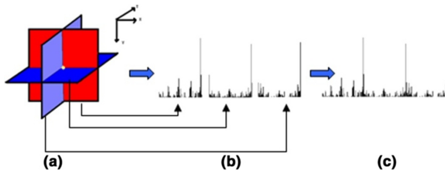
Figure 1 LBP from three orthogonal planes. (a) Three planes intersecting one pixel. (b) LBP histogram of each plane. (c) Concatenating the histograms (courtesy of [21]).
