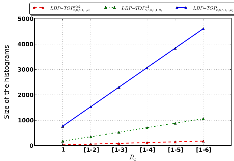
Figure 10 Evaluation of the histogram size when ( R_t ) is increased.
