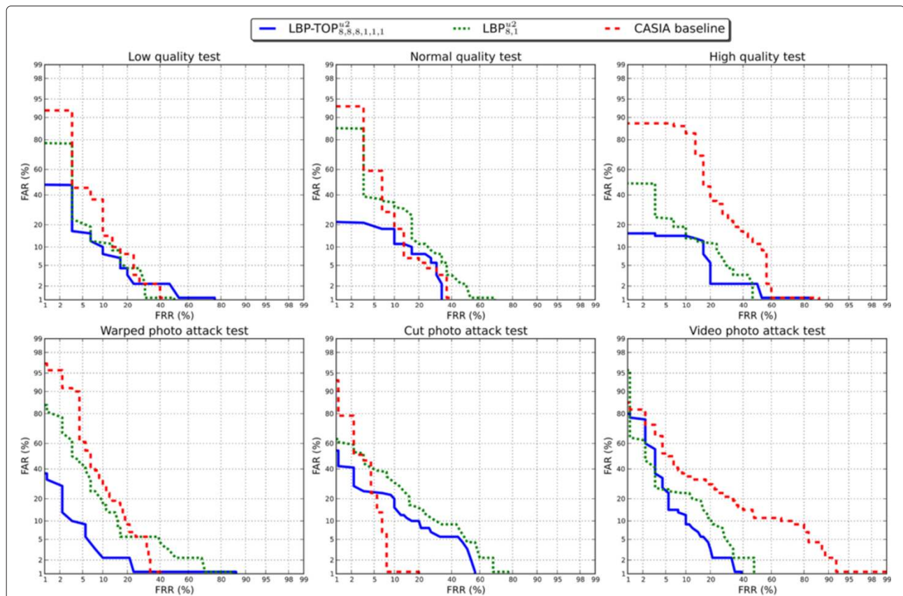
Figure 14 The different test protocols of the CASIA Face Anti-Spoofing Database. Performance of LBP-TOP_{8,8,8,1,1,1}^{u2} using the average of features compared to the DoG baseline method and LBP_{8,1}^{u2} .
