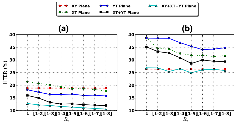
Figure 7 Evaluation of HTER (%) in each plane when multiresolution area ( R_t ) is increased. With LBP-TOP _{8,8,8,1,1,R_t}^{u2} and LDA classifier test set. (a) Replay-Attack Database. (b) CASIA Face Anti-Spoofing Database.
