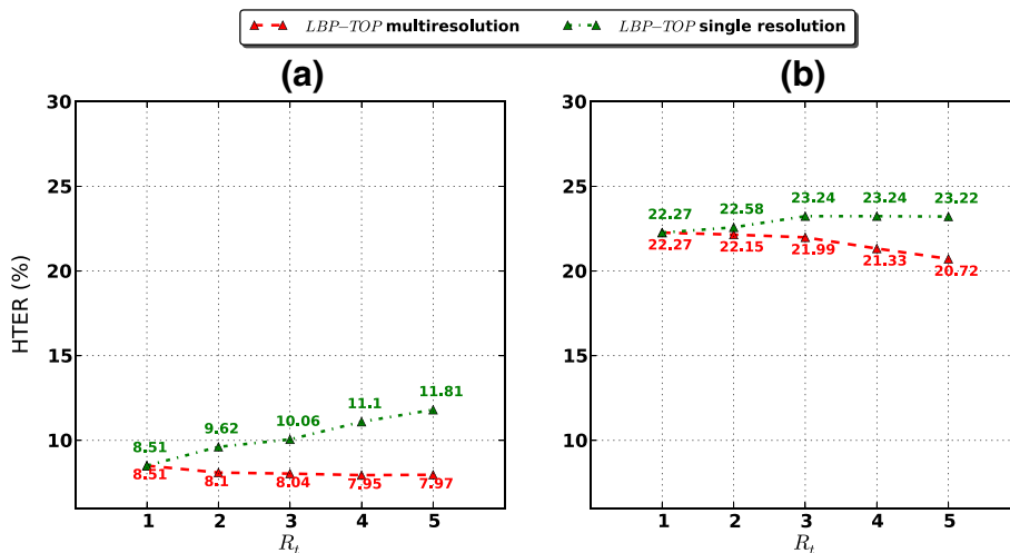
Figure 11 Evaluation of HTER (%) using LBP-TOP_{8,8,8,1,1,R_t}^{u2} with single resolution and multiresolution approach using SVM classifier. (a) Replay-Attack Database. (b) CASIA Face Anti-Spoofing database.
