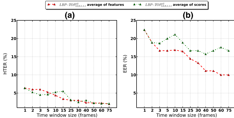
Figure 12 Access attempt-based evaluation. Different time window sizes were evaluated using mean of features and mean of scores with LBP-TOP u2 8,8,1,1,1 . (a) Replay-Attack Database (HTER %). (b) CASIA Face Anti-Spoofing Database (EER %).
