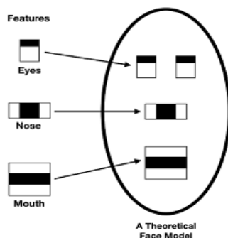
Fig.2. Haar Features
