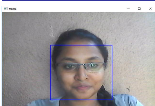
Fig.3. Face Detection
