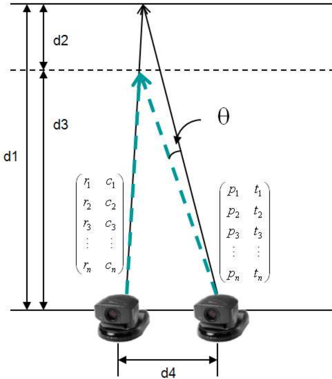
Figure 2.32. Calibration between static and PTZ cameras.
