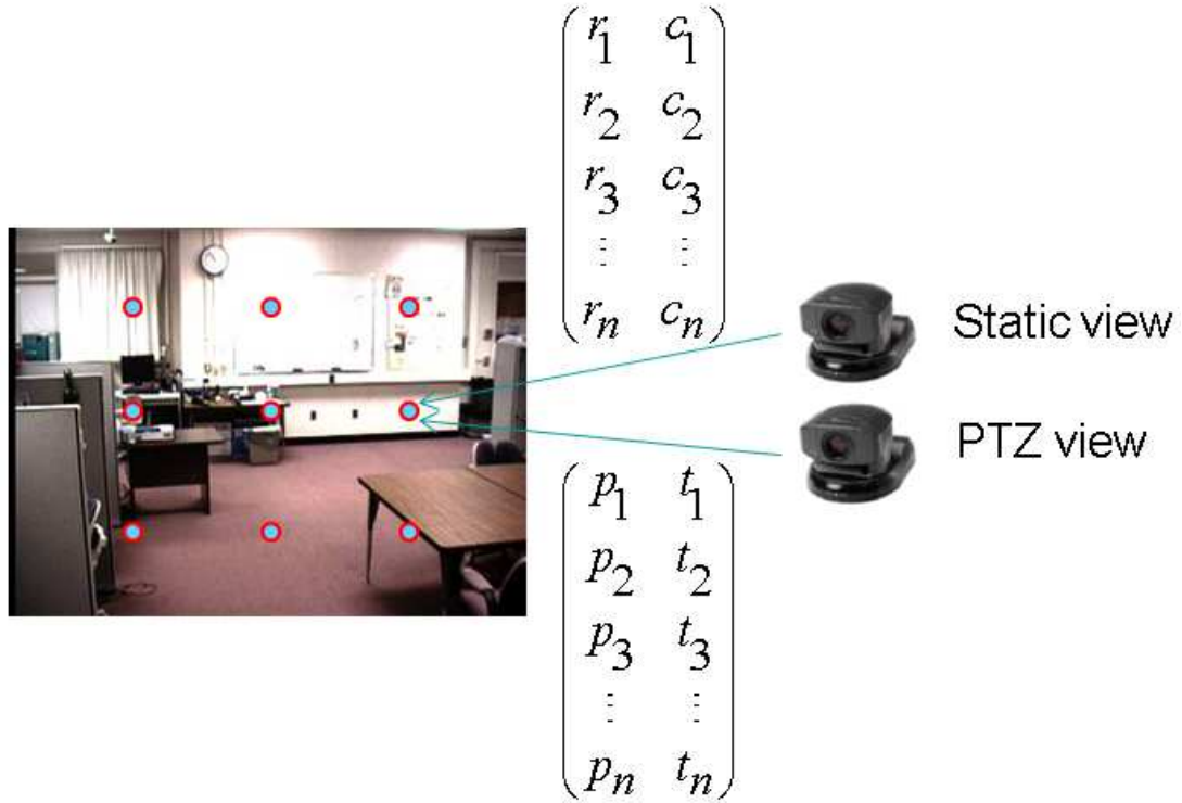
Figure 2.31. Schematic of camera calibration.
