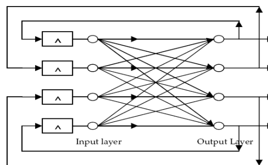
Figure 7. Recurrent Connected Network
