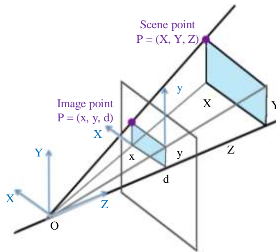
Fig. 7: Perspective transformation
