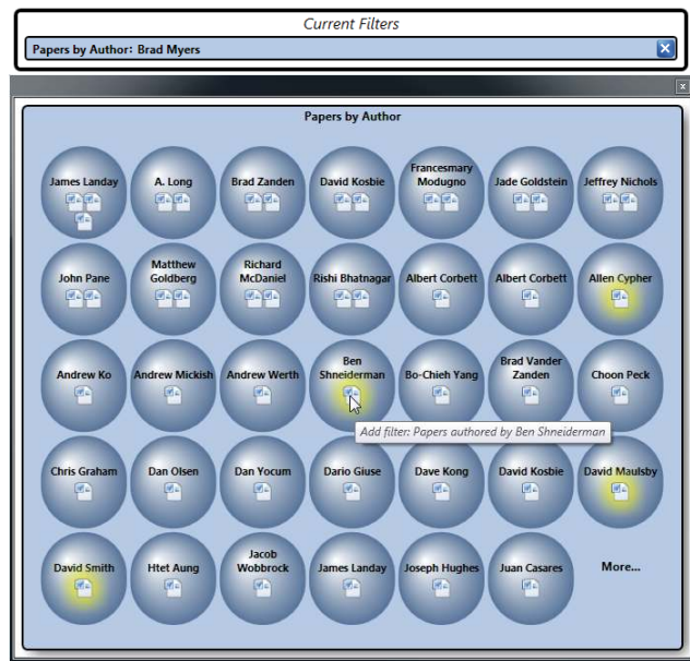
Figure 2. Flyout window for the “Papers by Author” facet with “Brad Myers” filter applied shows his co-authors. One particular paper is highlighted under four different co-authors on mouseover.
