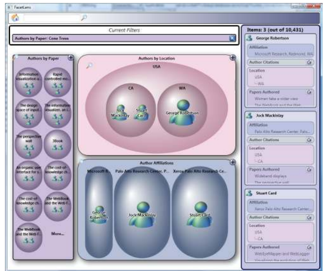
Figure 5. The metadata is shown for the three authors of the Cone Trees paper as a result of the pivot operation.
