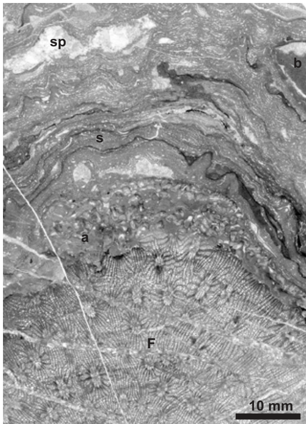
Figure 8: Domal stromatoporoid- Frechastraea association. Frechastraea pentagona colony (F) has first been thickly encrusted by auloporids (a). This latter have been covered by irregular laminar stromatoporoids (s) where sparitic cavities correspond to (small?) decayed sponges (sp). Stromatoporoids have also wrapped brachiopod shell (b) and other bioclasts. This is an uncommon case of growth because usually, stromatoporoids form only thin lamina like in bodies shown in pictures 11. Lambermont section, Unit B (bed 13/80).
