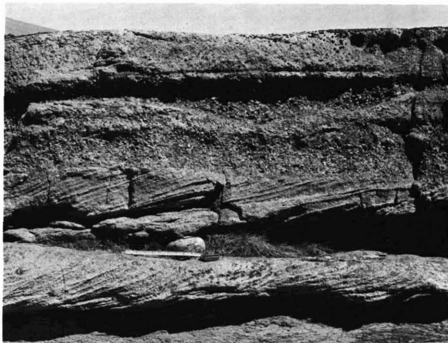
Figure 9 Pebbly sandstone facies, showing medium scale cross bedding. In isolation, this photograph could easily be confused with a photograph of fluvial gravels, but in fact is
