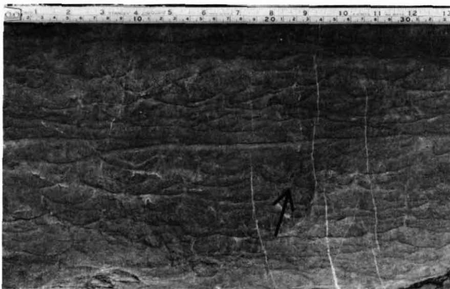
Figure 7 "Dish" structures, formed by rapid dewatering of a massive sandstone. Some of the dish edges curve upward into vertical
