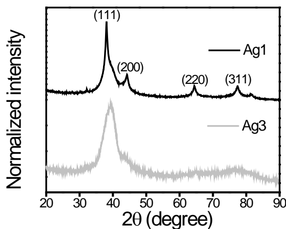
Figure 6. X-ray diffraction patterns of Ag1 and Ag3 silver nanoparticles. Source: The authors
