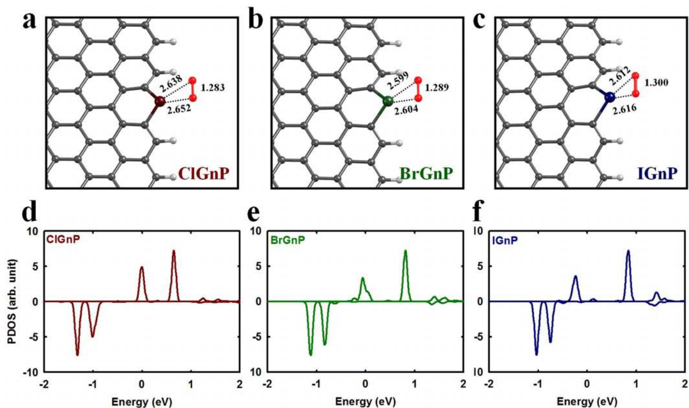
Figure 4 | The optimized O 2 adsorption geometries onto XGnPs, in which halogen covalently linked to two sp 2 carbons. (a) ClGnP; (b) BrGnP; (c) IGnP. The projected density of electronic states onto O 2 : (d) ClGnP; (e) BrGnP; (f) IGnP for the cases of corresponding (a), (b), and (c), respectively. In (a), (b) and (c), the O-O bond length and the shortest C-O bond are shown in angstroms.
