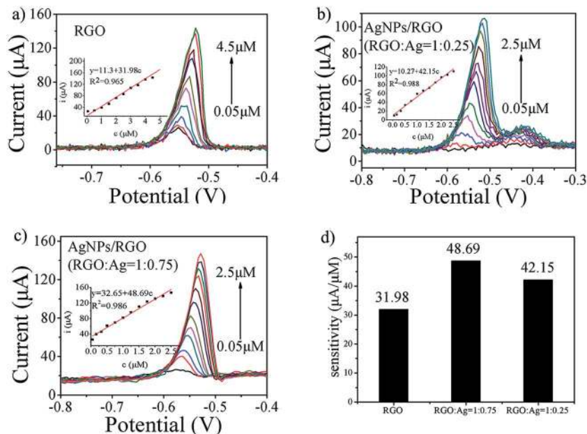
Fig. 4 (a–c) SWASV response toward \text{Pb}(\text{II}) detection on RGO : Ag = 1 : 0.25 and 1 : 0.75 modified MGCE electrodes in 0.1 M \text{HAC}-\text{NaAc} ( \text{pH} = 5.0 ) at the deposition potential of -1.0 V for 150 s. The potential step is 5 mV, the amplitude is 20 mV, and the frequency is 25 Hz. (d) Comparison between the sensitivity versus \text{Pb}(\text{II}) for the modified electrodes based on the different materials considered in this work.
