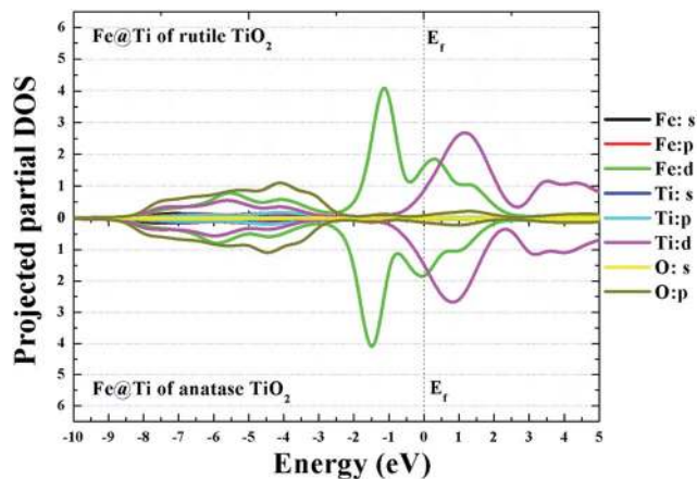
Fig. 10 DOSs for Fe replacing Ti in rutile and anatase \text{TiO}_2 .
