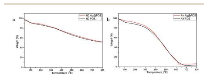
Fig. 7 TGA curves of (a) poly-dopamine spheres (PDS) and (b) poly-dopamine spheres loaded with silver nanoparticles (Ag@PDS).
