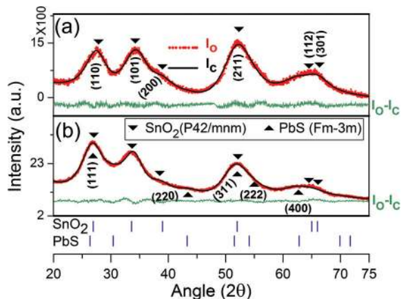
Fig. 2 Observed ( I_O ) and simulated ( I_C ) XRD patterns (indexed) of (a) SnO 2 NPs and (b) SnO 2 -PbS nanocomposites. The green lines represent I_O-I_C . Vertical markers corresponding to reflections from individual phases are shown in blue.
