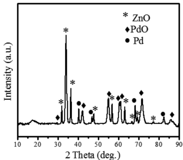
Fig. 3 X-ray diffractogram of the ZnO@PdO/Pd nanomaterial.
