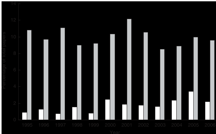
Fig. 2. The number of papers examining facilitation (open bars) and competition (closed bars) as a percentage of the total number of papers published in five leading plant ecology journals ( American Naturalist , Ecology , Journal of Ecology , Oikos and Oecologia ) between 1995 and 2006. Data obtained from ISI Web of Knowledge ( http://portal.isiknowledge.com/ ; 1 March 2007) using the search strings [(‘positive interaction*’ OR facilitation) AND plant*] or alternatively [(‘negative interaction*’ OR competition) AND plant*], specifying English language articles only. After Dormann & Brooker (2002).
