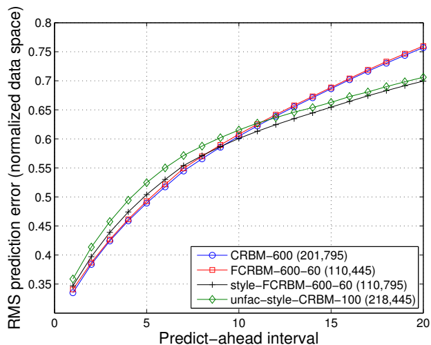
Figure 6. Prediction experiment. The number of free parameters are shown in parentheses. Error is reported in the normalized space in which the models are trained and is per-dimension, per-frame.
