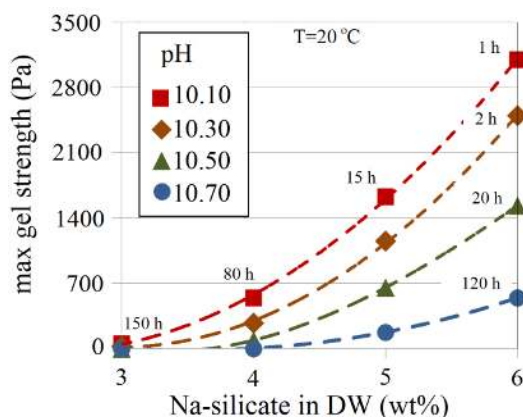
Figure 18. Maximum gel strength as a function of Na-silicate content and t_g . Corresponding t_{mgs} values are shown for different gelation times. pH values are presented in the graph for 6 wt% Na-silicate content with different gelation times and for the different Na-silicate contents with t_g = 1 min.
