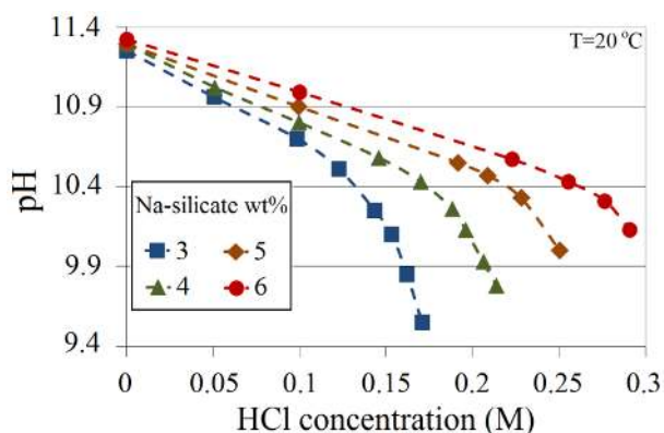
Figure 3. Corresponding pH for 3 wt%, 4 wt%, 5 wt% and 6 wt% Na-silicate solutions as a function of HCl concentration.
