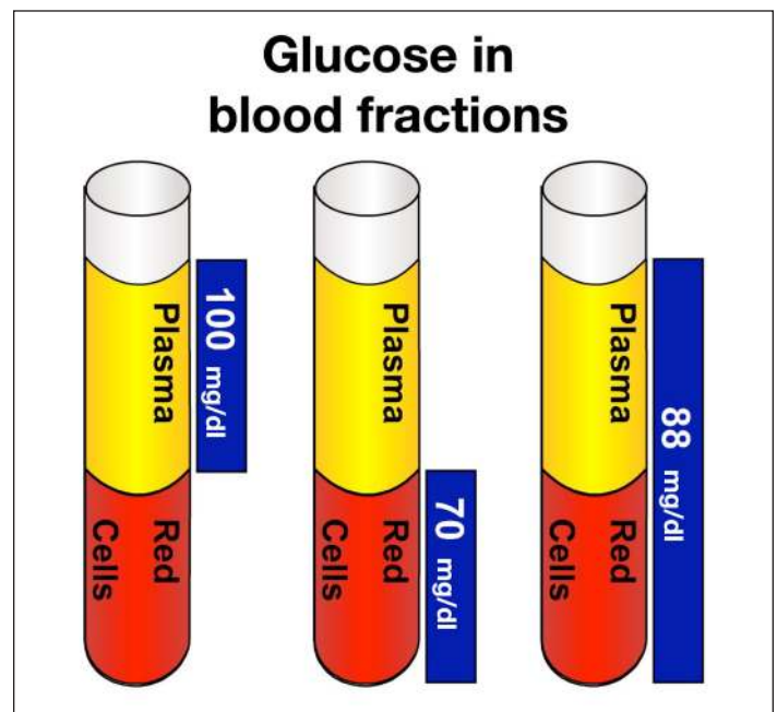
Figure 11. Glucose in erythrocytes is in equilibrium with plasma glucose but at lower levels. The total blood glucose, therefore, is dependent on the hematocrit.
