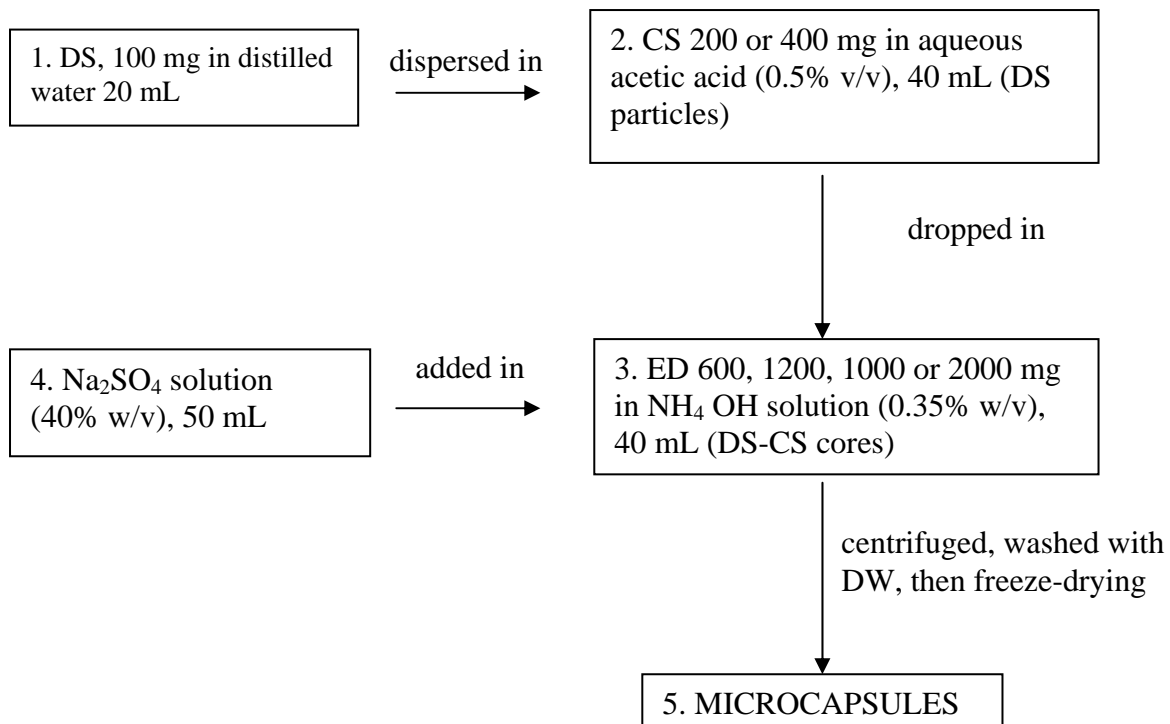
Figure 1. Microcapsules preparation process
