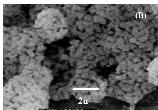
Figure 2. SEM micrographs of CS microcapsules (DS:CS:ED, 1:2:6) (A) 1000X and (B) 10000X magnification
