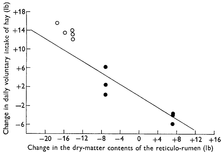
Fig. 2. Change, in the voluntary daily intake of hay by cows, caused by the removal of swallowed hay on isolated days (Expt 1, O), or by daily increases or decreases in the dry-matter contents of the reticulo-rumen (Expt 2, ●). The line represents the relationship expected when the removal or addition of 1 lb dry matter changes the voluntary intake of hay by 0.6 lb.
