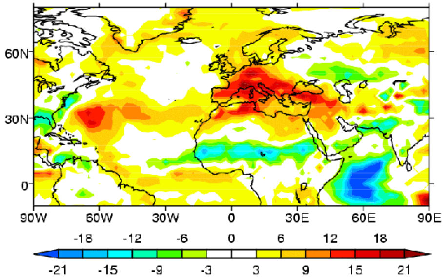
Figure 3 NOAA satellite-observed outgoing long-wave radiation (OLR) anomalies averaged over June-August 2003, calculated as departures from the 1979-1995 climatological average. Units are \text{Wm}^{-2} .
