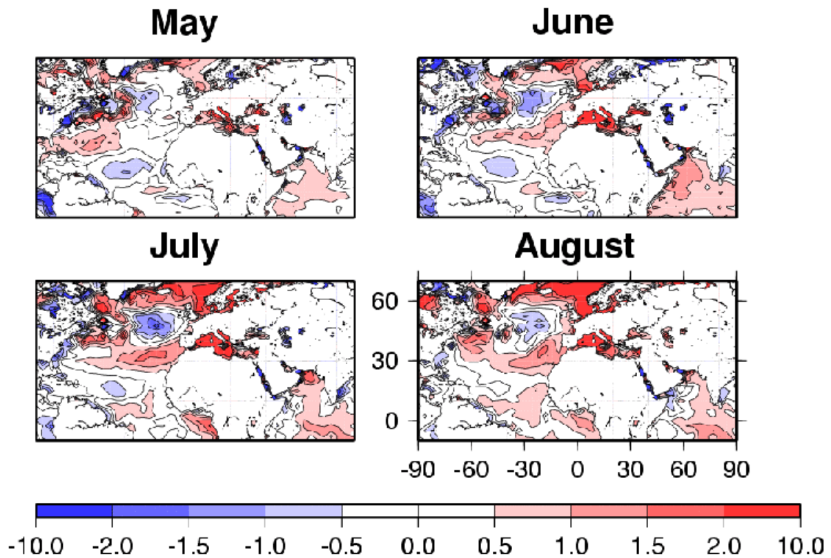
Figure 4 Monthly mean SST anomalies (skin temperature in ^{\circ}\text{C} ) for May to August 2003. The anomalies are calculated as the deviation of ECMWF operational analyses from the ERA-40 climatology for 1958-2001.
