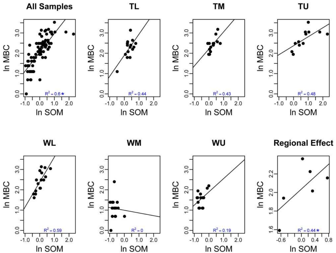
Figure 4. The \ln of the soil organic matter ( \mu\text{g SOM g}^{-1} dry soil) versus the \ln of the microbial biomass carbon ( \mu\text{g MBC g}^{-1} dry soil) for all of the samples (pane 1), at the six sites (panes 2–7), and regional effects (pane 8). Significant relationships have been noted for panes 1 and 8 (*) and a \neq in panes 2–7 indicates that the within site relationships are statistically different across sites (i.e. a local contextual effect was found).
