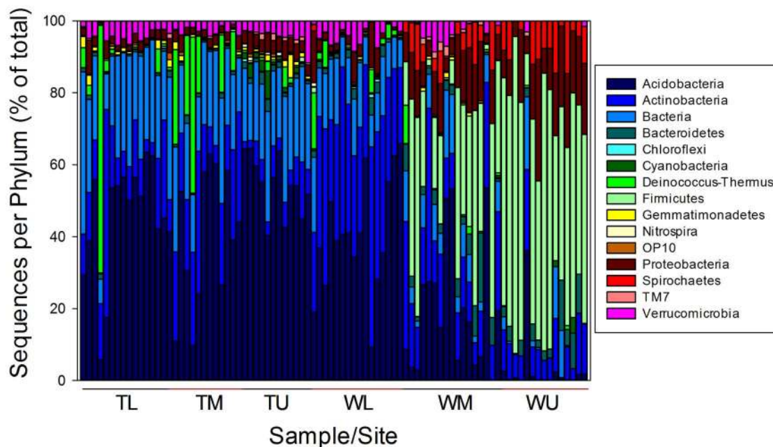
Figure 2. The phyla level taxonomy for each sample expressed as the percentage of the total sequences. doi:10.1371/journal.pone.0066103.g002
