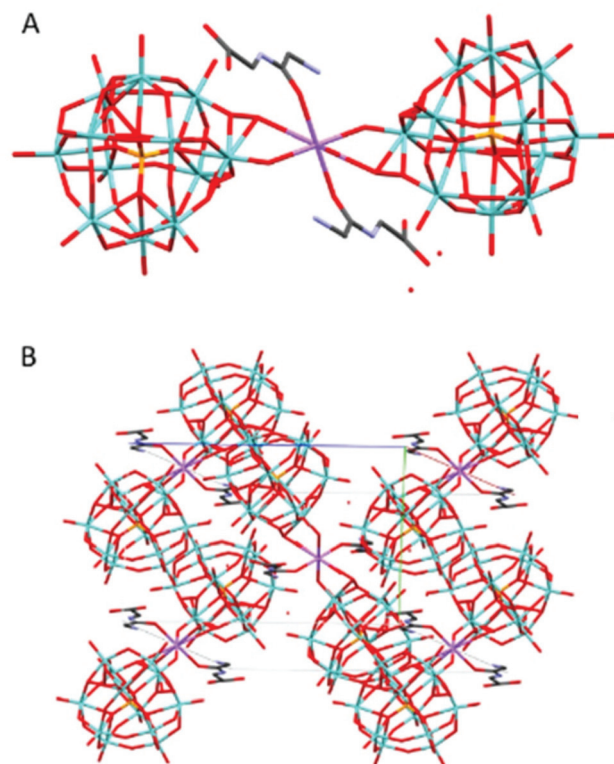
Fig. 7 The molecular (A) and crystal (B) structure of compound Na(HGlyGly) 2 (H 3 O) 3 [PMo 12 O 40 ] 2 \cdot 3H 2 O (7).
