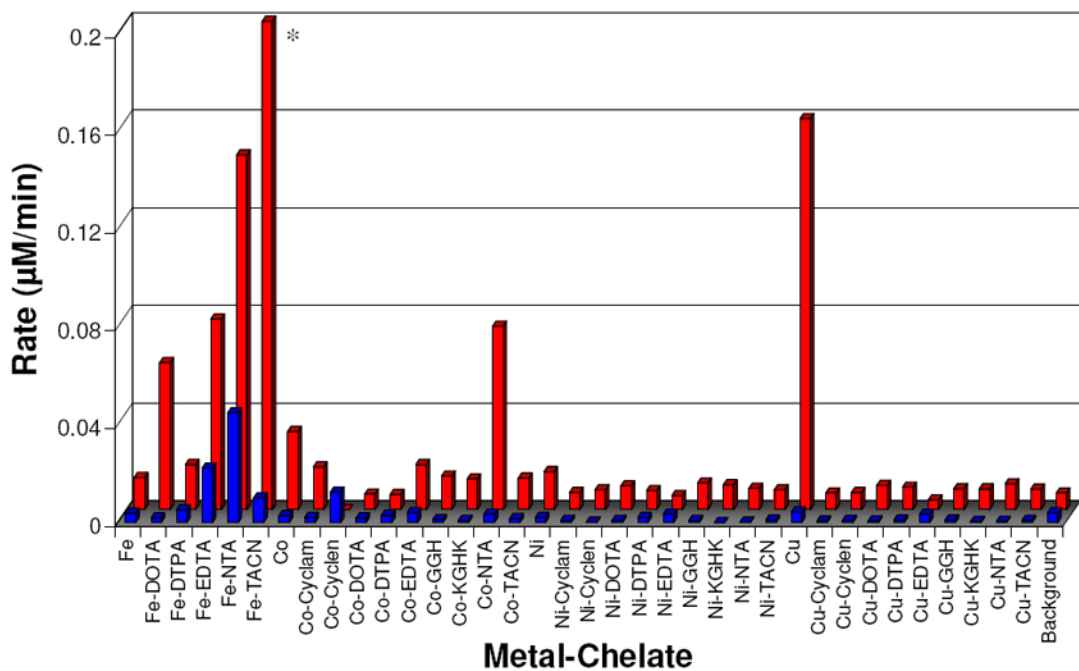
Figure 4. Summary of steady-state rates of TEMPO-9-AC monitored radical generation for each M-chelate/O 2 (front) and M-chelate/H 2 O 2 (rear) combination. * Fe-TACN/H 2 O 2 was observed to promote very rapid reaction relative to other catalysts, requiring stopped-flow measurements to determine an observed rate of 25.94 \pm 0.02 \mu\text{M}/\text{min} with the conditions used.
