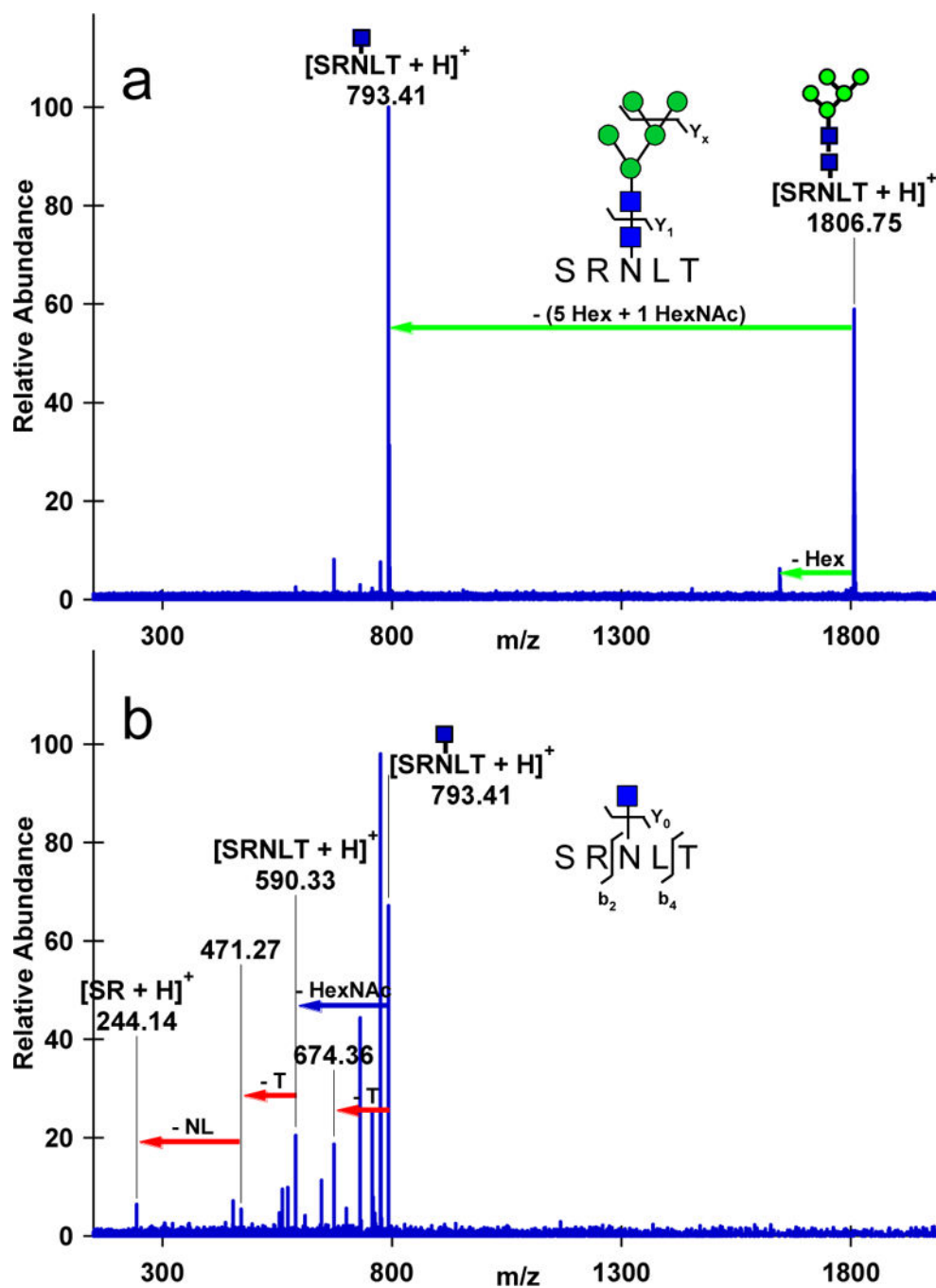
Figure 3. SORI-CID nano-ESI FT-ICR mass spectra; (a): MS/MS of protonated RNase B glycopeptide ^{58}\text{SRNLT}^{62} + \text{Man}_5 m/z 1806.75 (5 scans); (b): MS/MS/MS of the major product from (a), m/z 793.41 (50 scans).
