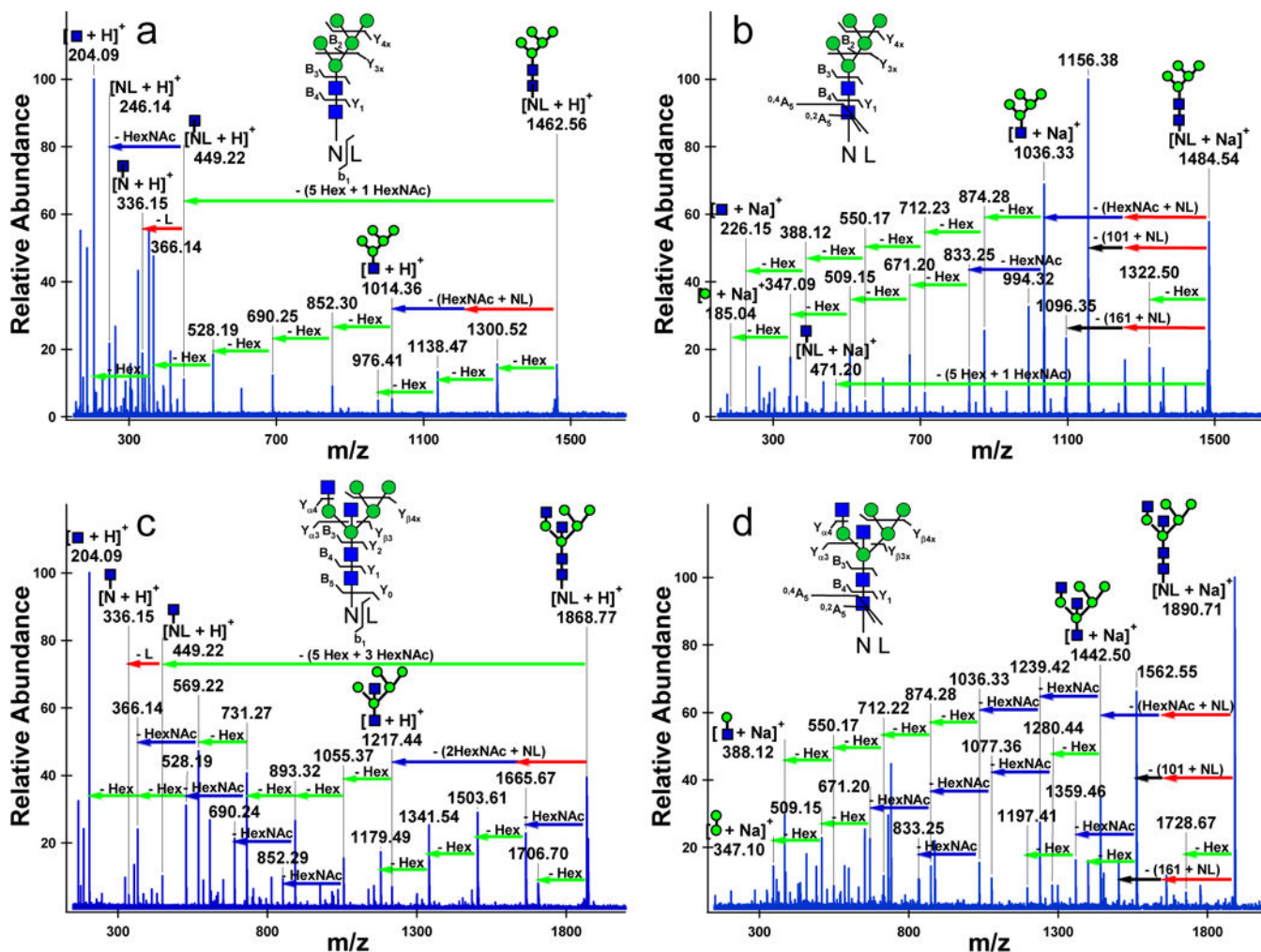
Figure 4. IRMPD nano-ESI FT-ICR mass spectra of glycopeptides without basic residues. The RNase B glycopeptide ^{60}\text{NL}^{61} + \text{Man}_5 ; (a): proton coordinated m/z 1462.56 (10 scans); (b): sodium coordinated m/z 1484.54 (10 scans). The CEA glycopeptide ^{292}\text{NL}^{293} + \text{HexNAC}_4\text{Hex}_5 (hybrid type glycan); (c): proton coordinated m/z 1868.74 (25 scans); (d): sodium coordinated m/z 1890.71 (10 scans).
