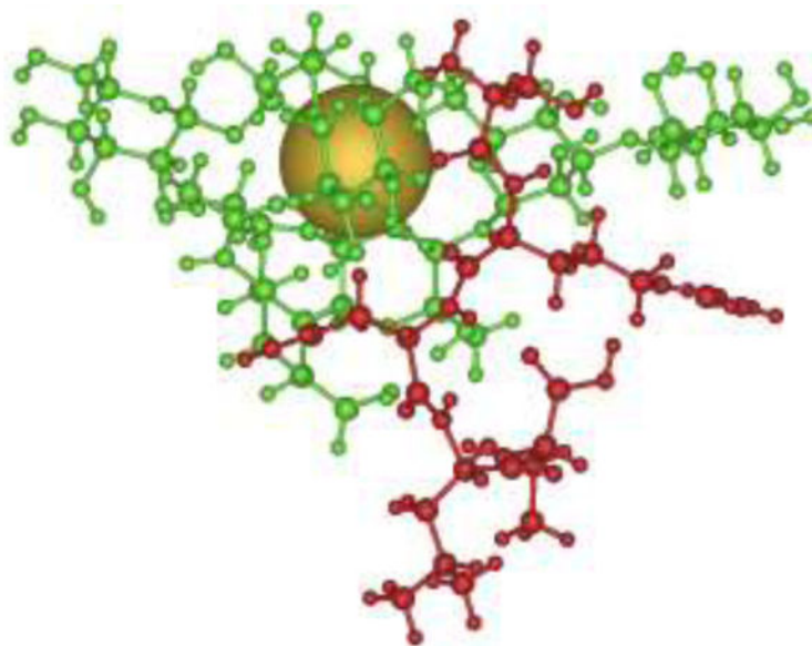
Figure 5. Simulated coordination of sodium cation to the RNase B glycopeptide ^{58}\text{SRNLT}^{62} + \text{Man5} . The sodium (yellow) is represented as space filling, while the glycan (green) and peptide (red) portions are represented as ball and stick. The sodium is coordinated in a multidentate fashion with the majority of the coordination stemming from the hydroxyl oxygens and little interaction with the peptide.
