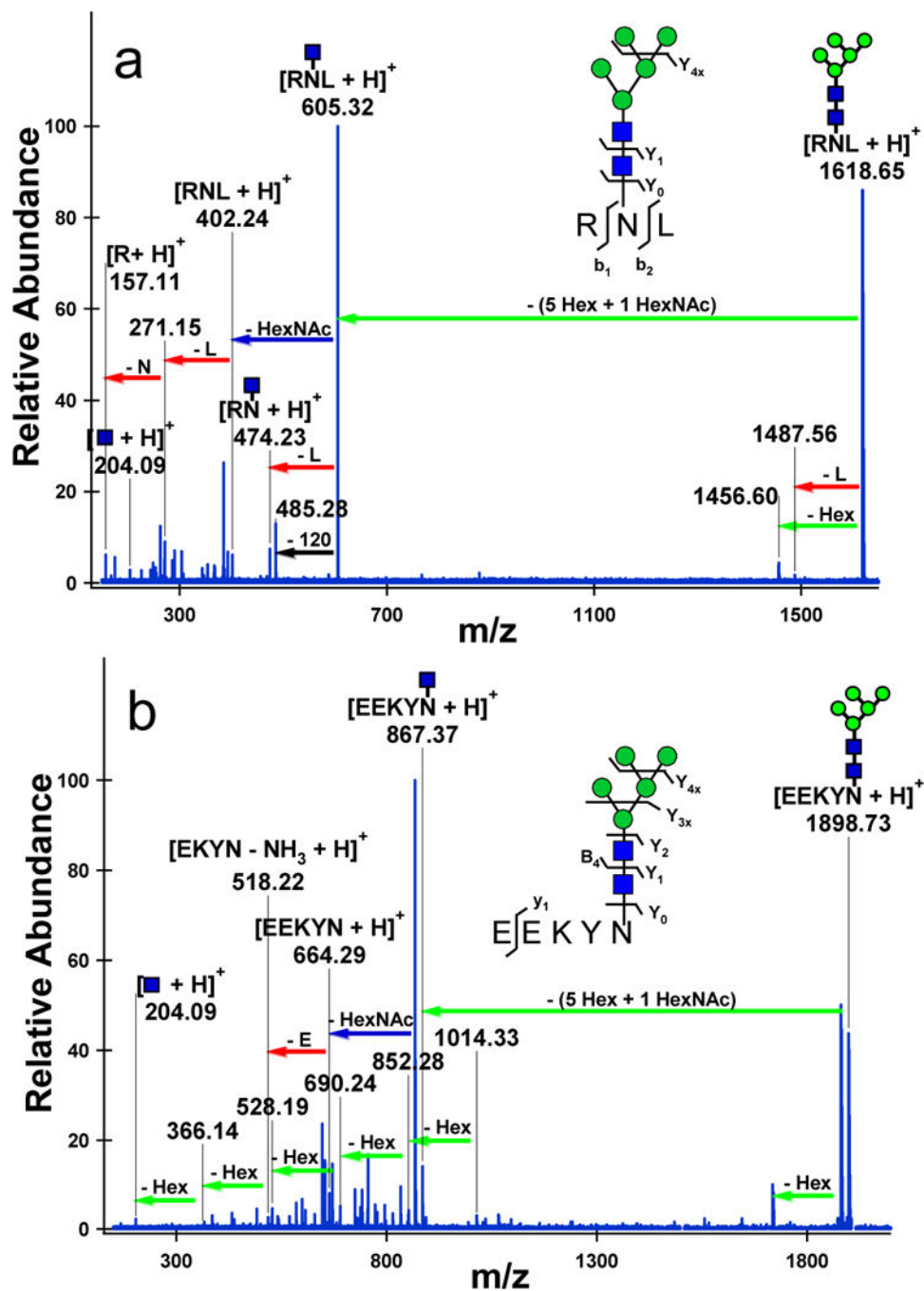
Figure 2. IRMPD nano-ESI FT-ICR mass spectra of proton coordinated glycopeptides yield similar fragmentation behavior; (a): RNase B glycopeptide ^{59}\text{RNL}^{61} + \text{Man}_5 m/z 1618.65 (10 scans); (b): CEA glycopeptide ^{288}\text{EEKYN}^{292} + \text{Man}_5 m/z 1898.73 (10 scans).
