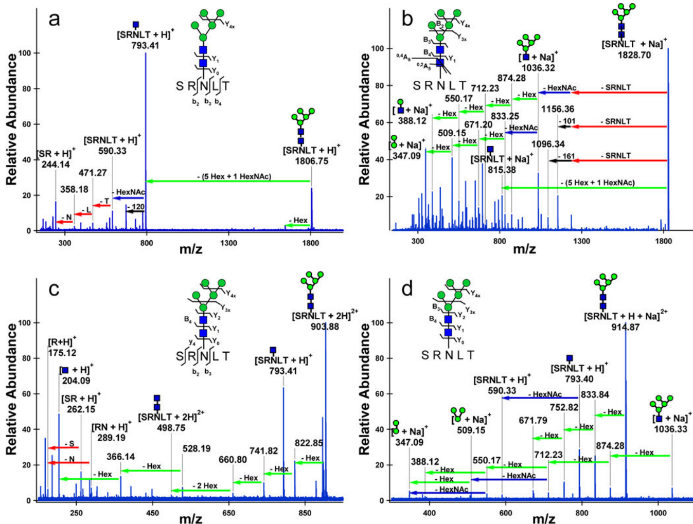
Figure 1. IRMPD nano-ESI FT-ICR mass spectra of the glycopeptide ^{58}\text{SRNLT}^{62} + \text{Man}_5 derived from RNase B with multiple coordinating ions: (a): singly charged proton coordinated glycopeptide m/z 1806.75 (5 scans); (b): singly charged sodium coordinated glycopeptide m/z 1828.70 (10 scans); (c): doubly charged doubly proton coordinated glycopeptide m/z 903.88 (5 scans); (d): doubly charged proton and sodium coordinated glycopeptide m/z 914.87 (15 scans).
