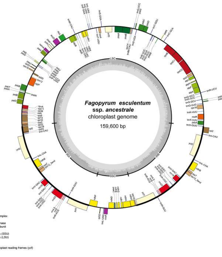
FIGURE 4 | Gene map of F. esculentum ssp. ancestrale chloroplast genome. The genes shown outside of the circle are transcribed clockwise, while those inside are counter clockwise.
