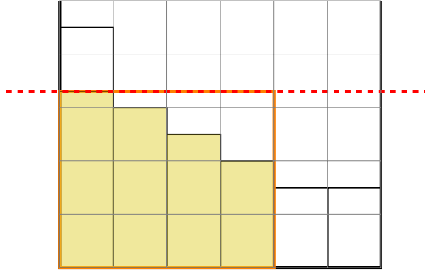
Fig. 3. Illustration of the function g . When n = 4 , g(\mathbf{h}) is the yellow area.
