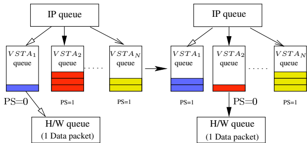
Figure 6: Queue Management.
