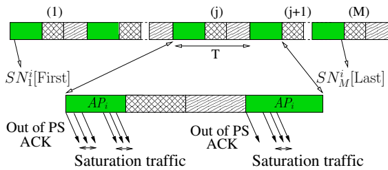
Figure 5: THEMIS estimators are based on local processing at MAC and PHY layer.
