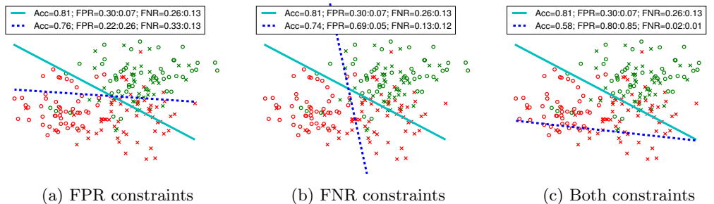
Figure 6: [Disparate mistreatment constraints] DM_{FPR} and DM_{FNR} have the same sign. Removing disparate mistreatment on FPR can potentially increase disparate mistreatment on FNR. Removing disparate mistreatment on both at the same time causes a larger drop in accuracy.
