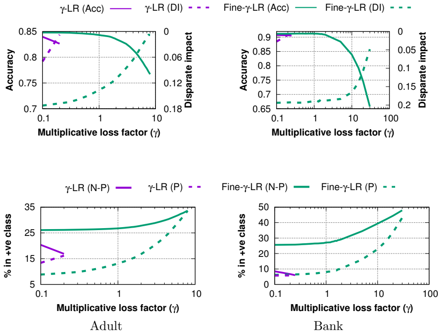
Figure 10: [Business necessity clause] Panels in top row show the accuracy (solid) and disparate impact (dashed) against \gamma . Panels in the bottom row show the percentage of protected (P, dashed) and non-protected (N-P, solid) users in the positive class against \gamma .
