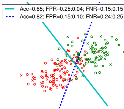
Figure 4: [Disparate mistreatment constraints] The figure shows the original decision boundary (solid line) and fair decision boundary (dashed line), along with corresponding accuracy and false positive rates for groups z = 0 (crosses) and z = 1 (circles). Fairness constraints cause the original decision boundary to rotate such that previously misclassified subjects with z = 0 are moved into the negative class (decreasing false positives), while well-classified subjects with z = 1 are moved into the positive class (increasing false positives), leading to equal false positive rates for both groups.
