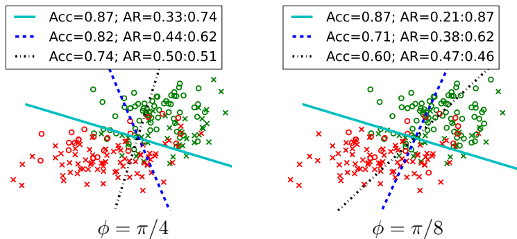
Figure 2: [Disparate impact constraints] Performance of different (unconstrained and constrained) classifiers along with their accuracy (Acc) and positive class acceptance rates (AR) for groups z = 0 (crosses) and z = 1 (circles). Green points represent examples with y = 1 and red points represent example with y = -1 . The solid lines show the decision boundaries for logistic regression classifiers without fairness constraints. The dashed lines show the decision boundaries for logistic regression classifiers trained to maximize accuracy under fairness constraints (Eq. (4.13)). Each column corresponds to a dataset with different correlation value between sensitive attribute values and class labels.
