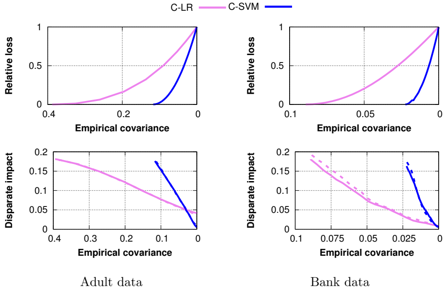
Figure 7: [Disparate impact constraints: Single, binary sensitive attribute] Panels in the top row show the trade-off between the empirical covariance in Eq. (4.2) and the relative loss with respect to the unconstrained classifier, for the Adult and Bank (training) datasets. Here each pair of (covariance, loss) values is guaranteed to be Pareto optimal by construction. Panels in the bottom row show the correspondence between the empirical covariance and disparate impact in Eq. (5.1) for classifiers trained under fairness constraints. Solid lines correspond to the training data whereas dashed lines correspond to the test data. The figure shows that a decreasing empirical covariance leads to higher loss but lower disparate impact. Moreover, the classifiers do not lead to “fairness overfitting”—in fact, the dashed lines for the Adult data are barely visible due to strong correspondance between the performance on the training and test sets.
