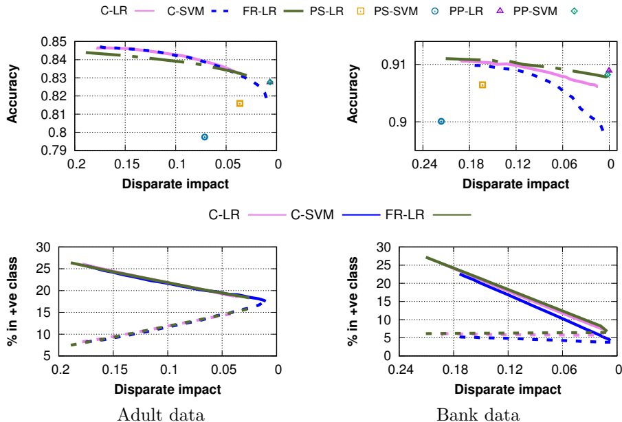
Figure 8: [Disparate impact constraints: Single, binary sensitive attribute] The figure shows the accuracy against disparate impact in Eq. 5.1 (top) and the percentage of protected (dashed) and non-protected (solid) users in the positive class against the disparate impact value (bottom). For all methods, a decreasing degree of disparate impact also leads to a decreasing accuracy. The post-processing technique (PP-LR and PP-SVM) achieves the best disparate impact-accuracy tradeoff. However, this technique as well as FR-LR use the sensitive feature information at decision time (as opposed to C-LR, C-SVM, PS-LR and PS-SVM), and would hence result in disparate treatment.
