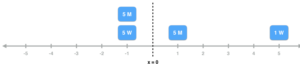
Figure 12: Covariance constraints may perform unfavorably in the presence of outliers. The figure shows a hypothetical dataset with just one feature ( x ) with values ranging from -5 to 5 . Data points belong to two groups: men (M) or women (W). Each box shows the number of subjects of from a certain group (M or W) with that feature value. The decision boundary is at x = 0 . The decision boundary covariance in this case is 0, yet the disparity in positive class outcome rates between men and women ( 0.5 for men and 0.17 for women) is very high. This situation is caused by one woman with feature value 5 —this outlier point cancels out the effect of five normal examples (W with feature value -1 ) while computing the covariance.
