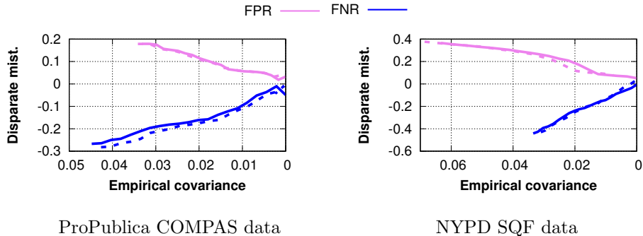
Figure 11: [Disparate mistreatment constraints] The figure shows the effect of applying Our method sen to limit disparate mistreatment with respect to false positive rate and false negative rate, as defined by Eqs. (5.2) and (5.3), respectively. Each type of constraint is applied separately. The plots show the correspondence between the empirical covariance (for each constraint type) and disparate mistreatment caused by the classifiers trained under fairness constraints on ProPublica COMPAS (left) and NYPD SQF (right) datasets. Solid lines correspond to the training data whereas dashed lines correspond to the test data. The figure shows that a decreasing empirical covariance leads to lower disparate mistreatment. Moreover, the statistics for training and test sets show a close correspondence, meaning that the constraints do not seem to be overfitting on the training data.
