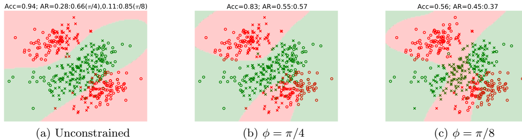
Figure 3: [Disparate impact constraints] Decision boundaries for SVM classifier with RBF Kernel trained without fairness constraints (left) and with fairness constraints (middle and right) on two synthetic datasets. Also shown are the classification accuracy (Acc) and acceptance rate (AR) for each group.
