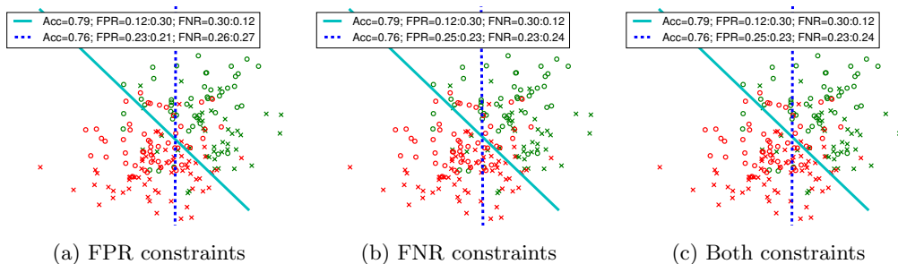
Figure 5: [Disparate mistreatment constraints] DM_{FPR} and DM_{FNR} have opposite signs. Removing disparate mistreatment on FPR can potentially help remove disparate mistreatment on FNR. Removing disparate mistreatment on both at the same time leads to very similar results.
