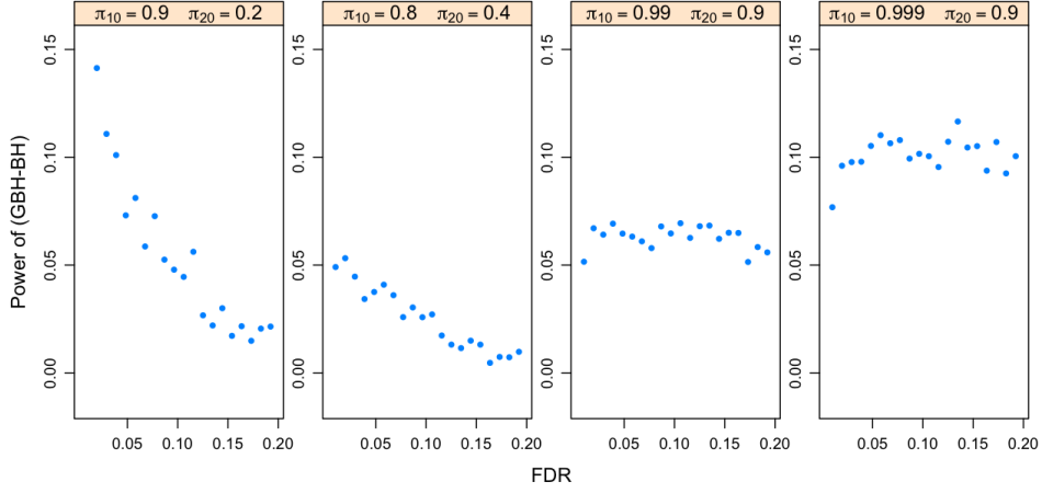
Figure 4: Power differences of the oracle BH and GBH procedures for p -values with the PRDS property. The p -values are generated based on model (4.1) with \xi_1 = \xi_2 = 0.5 and n = 10,000 for each group. Each panel corresponds to one combination of \pi_{q,0} 's for two groups.
