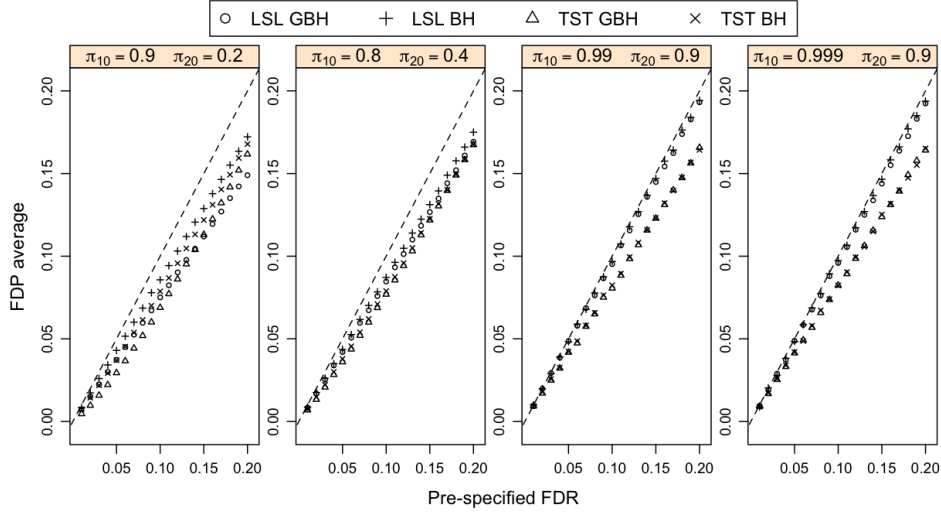
Figure 5: Comparison of the average FDP and the pre-specified FDR for the adaptive BH and GBH procedures. The dash line is the 45-degree line. The p -values are generated on model (4.1) with \xi_1 = \xi_2 = 0 and n = 10,000 for each group. Each point of the FDP is the average of 200 iterations.
