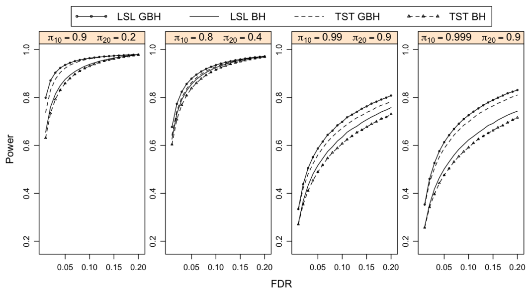
Figure 6: Power curves of the adaptive BH and GBH procedures for independent p -values. The p -values are generated based on model (4.1) with \xi_1 = \xi_2 = 0 and n = 10,000 for each group. Each panel corresponds to one combination of \pi_{g,0} 's for two groups.
