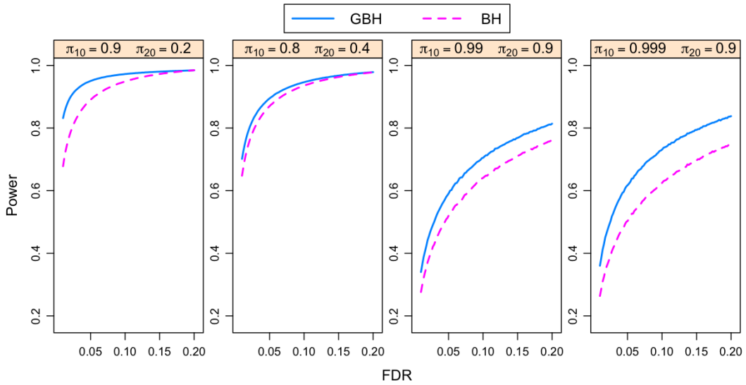
Figure 3: Power curves of the oracle BH and GBH procedures for independent p -values. The p -values are generated based on model (4.1) with \xi_1 = \xi_2 = 0 and n = 10,000 for each group. Each panel corresponds to one combination of \pi_{g,0} 's for two groups.
