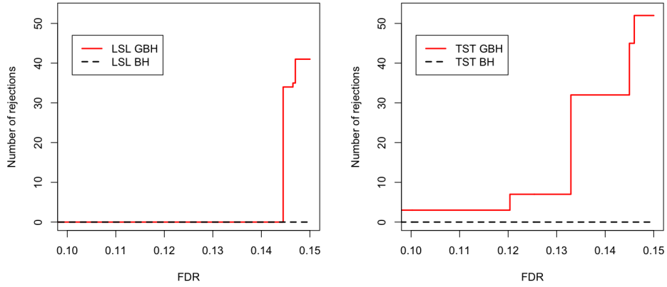
Figure 2: Breast cancer study, 9,492 genes. The plots show the number of genes detected by the adaptive BH and GBH procedures using Gene Ontology grouping. Left panel: the LSL method. Right panel: the TST method. Data from van't Veer et al (2002).
