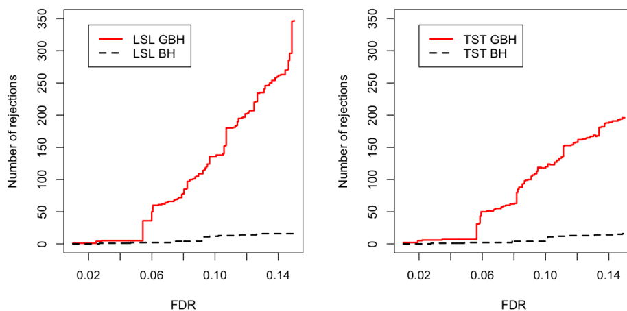
Figure 1: Breast cancer study, 24,184 genes. Plot shows the number of signals detected by GBH and BH procedures versus pre-specified FDR level. Left panel: adaptive LSL GBH procedure. Right panel: adaptive TST GBH procedure. Details for LSL and TST approaches are in section 2.3. Genes are assigned into six groups using k -means clustering. Data from van't Veer et al (2002).
