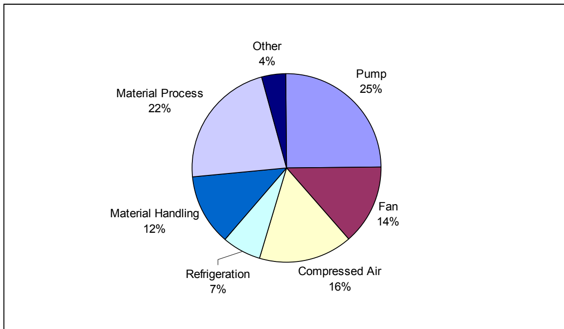
Figure 1: Motor Systems Energy End-Use (Source: Nadel et al. 2002)
