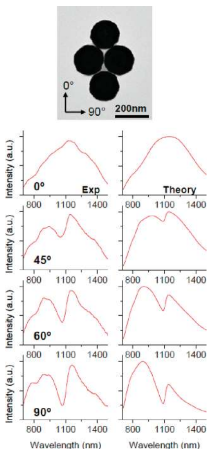
FIGURE 2. Scattering spectra of the quadrumer. TEM image and spectra of an asymmetric quadrumer. The orientation angles of the incident electric field relative to the cluster are shown in the TEM image. The experimental spectra show a Fano minimum at 1080 nm that varies with orientation angle and is strongest at 90°. The calculated spectra also show a Fano minimum with a similar resonant wavelength and dependence on orientation angle.
