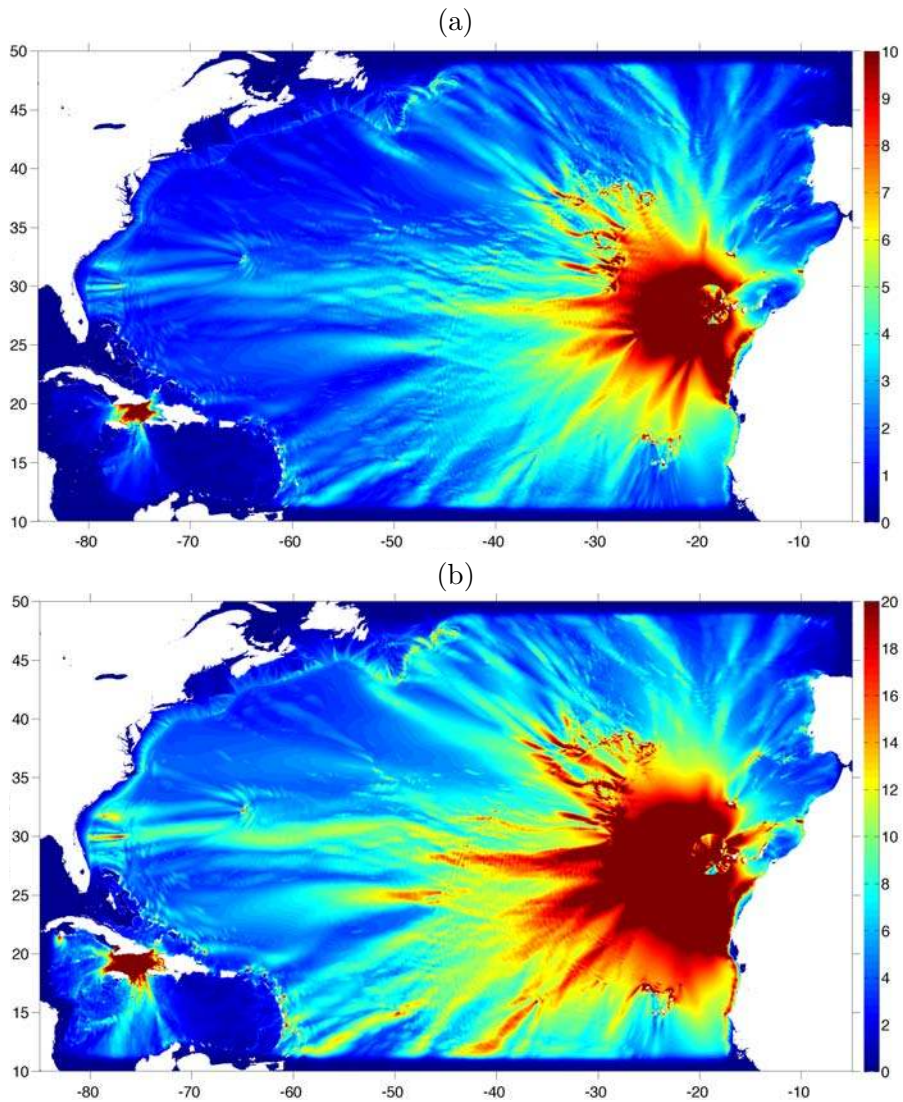
Figure 9. Maximum envelope of surface elevation (color scale in meter) computed with FUNWAVE-TVD in 1 arc-min Atlantic Ocean basin grid for the tsunami generated by the: (a) 80 km 3 ; and (b) 450 km 3 , CVV flank collapse scenarios. Axes are Long. E. (deg.) and Long. N. (deg.). [Note that both figures are plotted with a different color scale. Also note the large elevations, in both cases, west of Haiti and south of Cuba are an artifact of numerical simulations; more accurate simulations and details of the extreme CVV scenario impact in this area can be found in Grilli et al. (2015a).]
