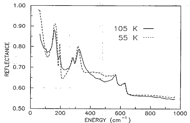
FIG. 1. Reflectance of \text{YBa}_2\text{Cu}_3\text{O}_7 in the normal state (solid curve) and superconducting state (dashed curve).
