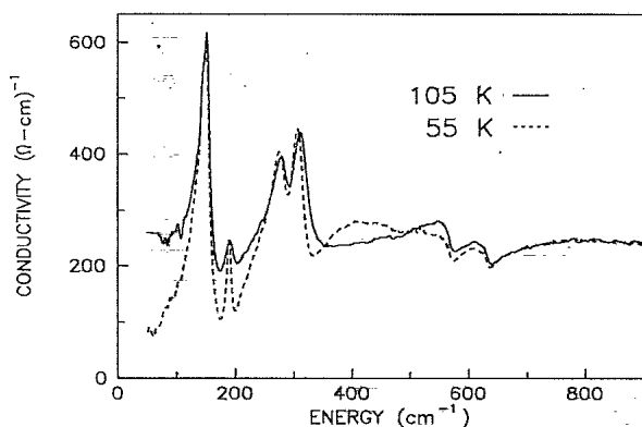
FIG. 2. The frequency-dependent conductivity of \text{YBa}_2\text{Cu}_3\text{O}_7 in the normal state (solid curve) and superconducting state (dashed curve). We associate the region of depressed conductivity below 200 \text{cm}^{-1} with the superconducting energy gap. The sharp peaks are due to phonons, the peaks at 279 and 312 \text{cm}^{-1} seem to be coupled to the electrons that participate in the superconducting transition.
