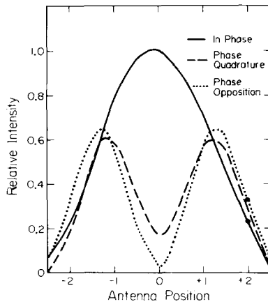
FIG. 5. Array images of two pinholes with varying relative phases. The points between the sampled antenna values were recovered by the standard sincfunction interpolation of sampling theory (Ref. 14 pp. 21–25). During the measurements, the bond on the antenna at +2 failed, and two data points were lost. To allow us to plot the entire curve, we filled in these two data points (solid circles) by symmetry.
