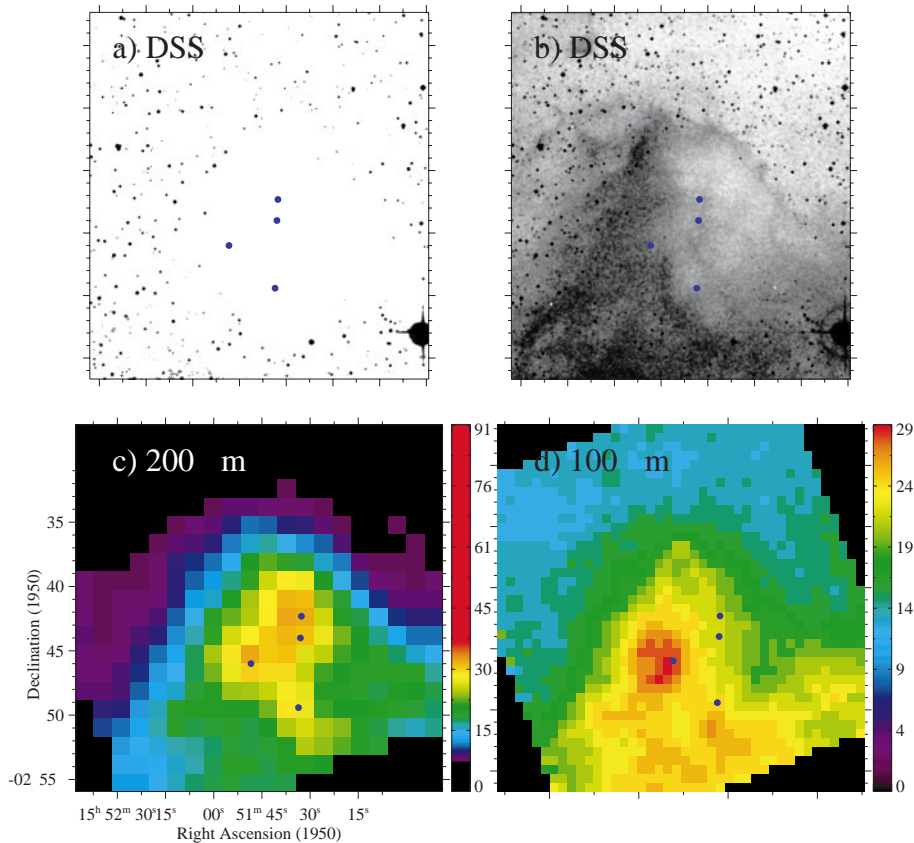
Fig. 1. Optical red Digitized Sky Survey (DSS) ( a ), ( b ), 200 \mu\text{m} ( c ) and 100 \mu\text{m} ( d ) images of L 183. The four unresolved sources are marked as blue dots; for identification see Fig. 3. a ) Digitized Sky Survey red plate. The image is scaled to best show the opaque core of the cloud. b ) Digitized Sky Survey red plate. The image is scaled to best show details of faint surface brightness. c ) False-colour image of 200 \mu\text{m} surface brightness. The colour scale is in units of \text{MJy sr}^{-1} . d ) False-colour image of 100 \mu\text{m} surface brightness. Zodiacal light of 4.0 \text{ MJy sr}^{-1} has been subtracted. The colour scale is in units of \text{MJy sr}^{-1} .
