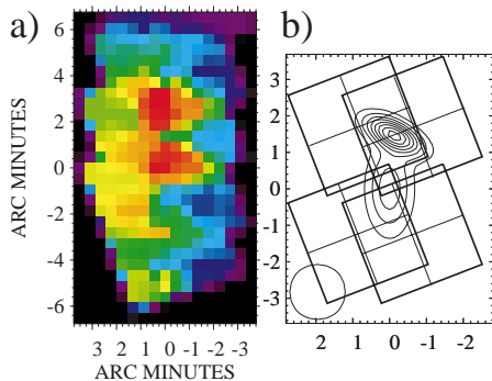
Fig. 2. a ) Map made from the 200 \mu\text{m} stripe scan data. The pixel size is 30'' . We note that this map is just to illustrate that the two continuum sources detected by Ward-Thompson et al. (1994, 2000) can be detected as separate sources in the stripe scan data. The details in this map are smaller than the actual resolution of the stripe scan data. b ) The model at 200 \mu\text{m} used to derive the fluxes of FIR 1 and FIR 2. The positions and sizes of the sources are those given by Ward-Thompson et al. (1994, 2000). The inclined boxes show the locations of the 2 \times 2 pixel C200 detector array in the North-South stripe scan. The contours of the continuum sources go from 0.8 to 6.4 in steps of 0.8 \text{ Jy pixel}^{-1} . The \text{FWHM} of the ISO beam at 200 \mu\text{m} is shown at lower left hand corner. The center position in both maps is the position of FIR 2 (see Table 3).
