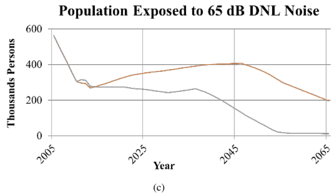
Fig. 1 Best and worst case fleet-level future scenarios for: (a) total fuel burn in billion kg; (b) takeoff NO_x in million kg; and (c) thousands of persons exposed to 65 dB DNL noise for 55 airports across the US.
