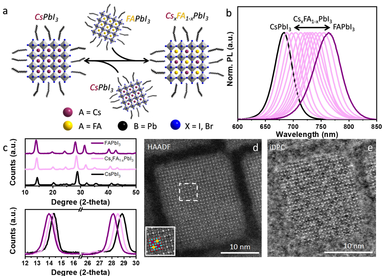
Figure 1. a) Schematic illustration of the formation of double-cation perovskite ( \text{Cs}_x\text{FA}_{1-x}\text{PbI}_3 ) NCs through reversible cation exchange by mixing \text{CsPbI}_3 and \text{FAPbI}_3 perovskite NCs. b) Normalized PL spectra of \text{CsPbI}_3 , \text{FAPbI}_3 and \text{Cs}_x\text{FA}_{1-x}\text{PbI}_3 NCs obtained by cation exchange. The emission wavelength of the mixed-cation NCs is tunable between those of the individual pure A-cation compositions. c) XRD diffraction pattern of \text{CsPbI}_3 , \text{FAPbI}_3 and \text{Cs}_x\text{FA}_{1-x}\text{PbI}_3 NCs obtained by cation exchange. In the bottom panel, the enlarged spectra evidence the peak shift that confirms the mixed cation composition. d, e) Representative high resolution HAADF-STEM (d) and integrated differential phase contrast (iDPC)-STEM (e) images of \text{Cs}_{1-x}\text{FA}_x\text{PbI}_3 NCs (PL peak at 725 nm). The uniform intensity in the HAADF-STEM image indicates that there is no segregation of the two cations in the lattice. Due to the mix of Cs and FA, the intensity of the A-site atomic columns is very low and hardly detectable in the HAADF image. However, the phase contrast in the iDPC image enables visualization of the Cs atoms. The overlay in the inset of panel (d) indicates the atom column position of Cs (purple), FA (yellow), Pb (red) and the halide (blue) in the perovskite structure. The Cs and FA cations are randomly mixed.
