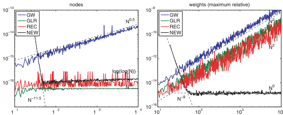
FIG. 2.1. Observed error in computing Gauss-Legendre nodes and weights. GW uses the dgauss routine from the ORTHPOL library [18], REC is glfixed from the GSL library [14], GLR is a Fortran implementation supplied by the authors of [23], and NEW is a MATLAB implementation of the algorithm presented in this paper. The C and Fortran codes are interfaced with MATLAB via MEX files. See Figure 4.3 for analogous plots of quadrature error and computational time.
