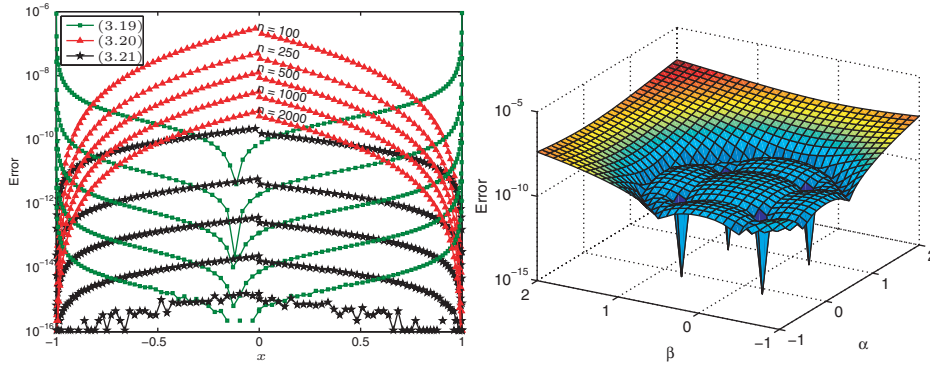
FIG. 3.6. Left: Error in approximations (3.19)–(3.21) for the roots of P_n^{(0.1,-0.3)}(x) , with n = 100, 250, 500, 1000, 2000 (descending). Here the crossover between the interior approximation (3.19) and Olver’s “boundary” approximation (3.21) doesn’t occur until x \approx 0.1 . Right: Error in approximation (3.21) for the roots of P_{100}^{(\alpha,\beta)}(x) for \alpha, \beta \in [-.9999, 2] . Although the accuracy degrades outside of the interval [-1/2, 1/2] , it is still sufficient for convergence of the Newton iteration.
